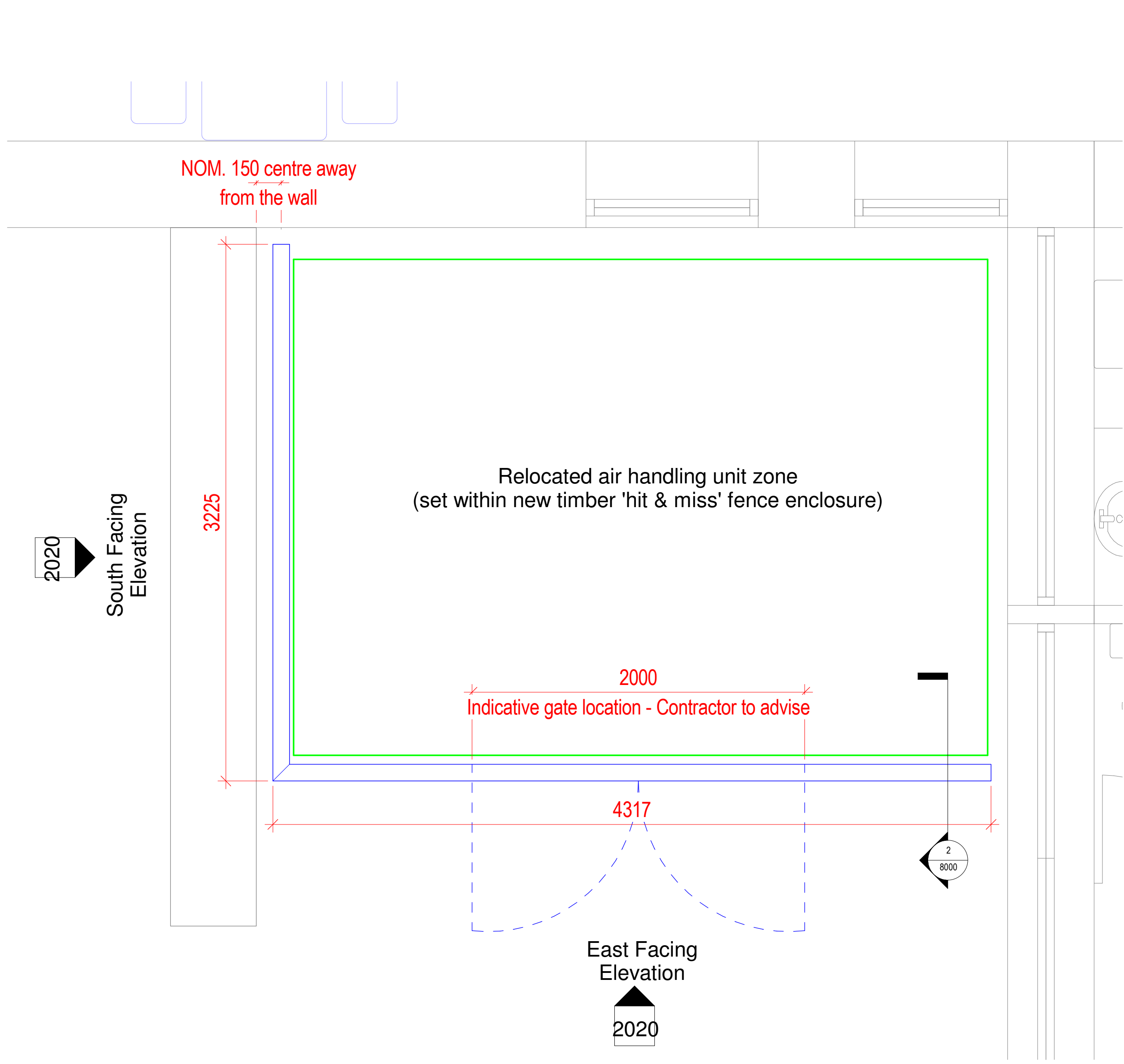
00 - Ground Floor - Plant Enclosure 1 : 20
