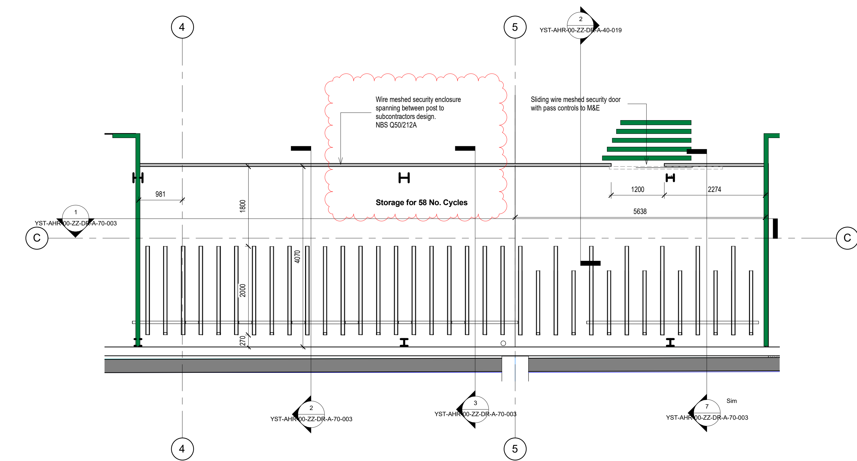
4 Basement Cycle Parking Area 1 : 50
