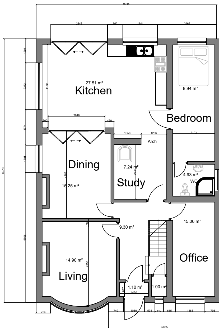
1 — Proposed Ground Floor Plan 1/100
