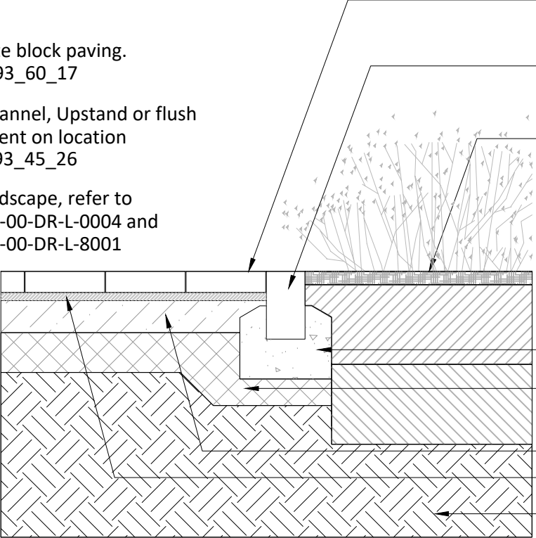
8004 10 Section: Paving with flush kerb and planting 1:20
