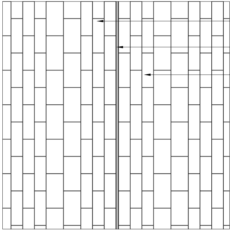
8004 03 Plan: Paving with slot drain 1:20
