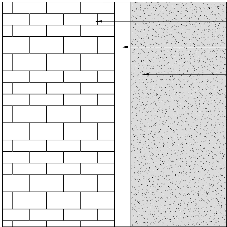
8004 05 Plan: Paving to resin bound gravel with flush kerb 1:20
