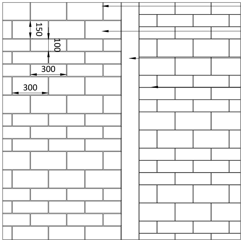
8004 01 Plan: Rigid paving to flexible paving 1:20
