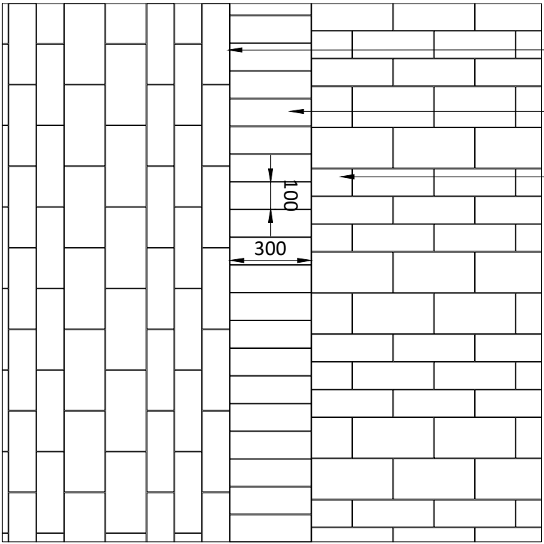
8004 11 Plan: Change of direction paving interface 1:20
