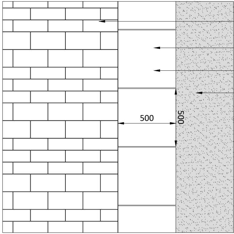
8004 07 Plan: Paving to resin bound gravel with paving trim 1:20
