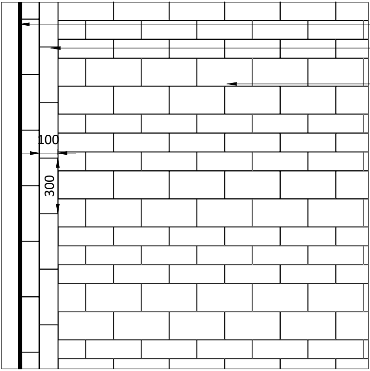
8004 15 Plan: Paving to building interface 1:20
