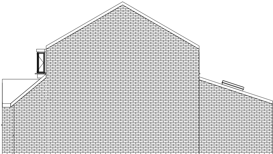
4 Right Proposed 1 : 100
