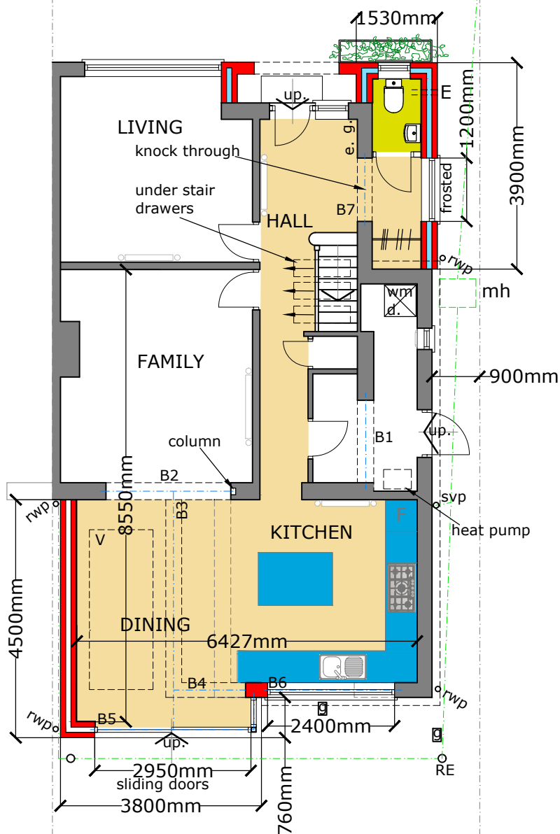
GROUND FLOOR
