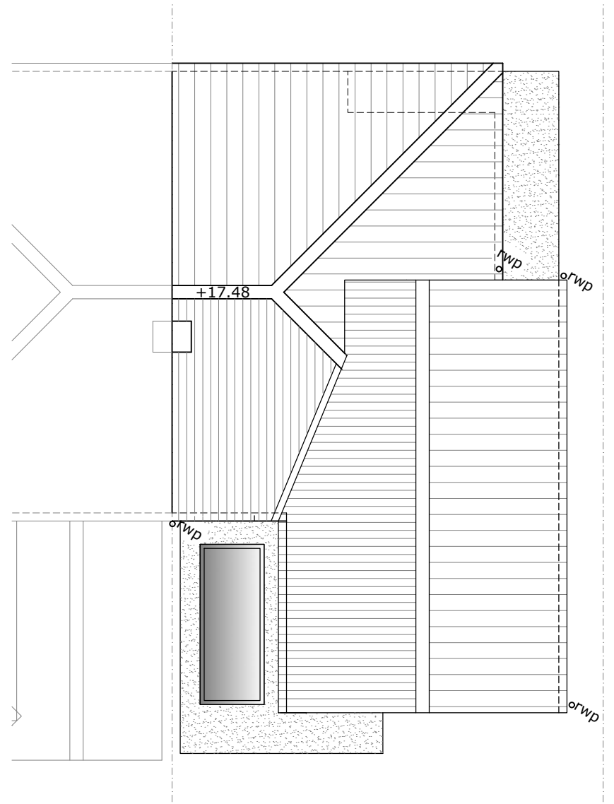
ROOF PLAN
