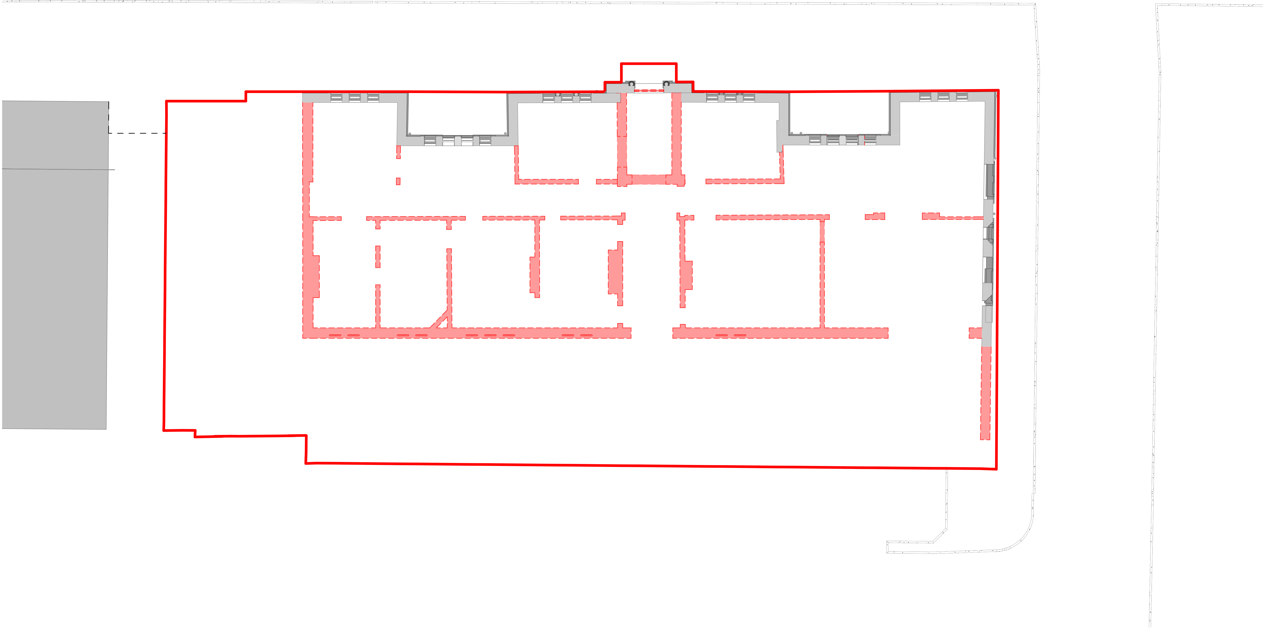
Ground Floor Demolition Plan 1 : 100
