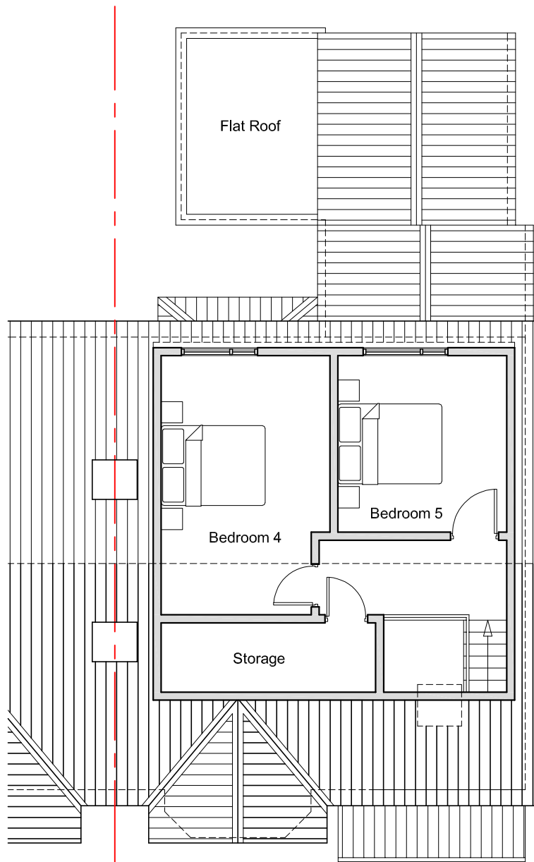
Proposed Loft Plan 1:100
