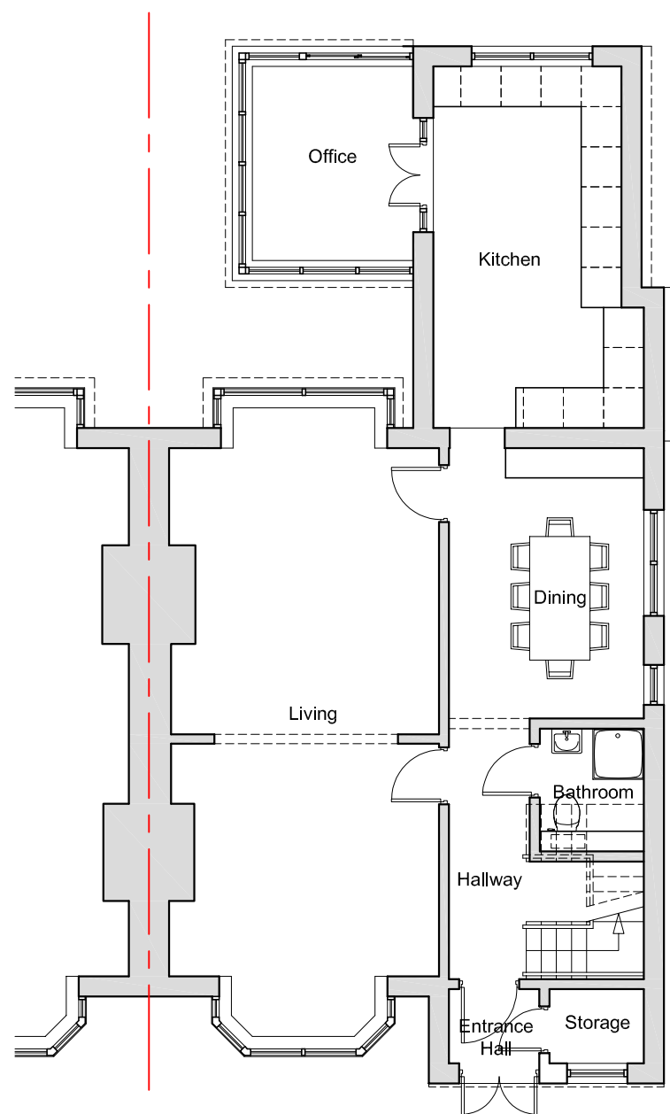
Proposed G/F Plan 1:100
