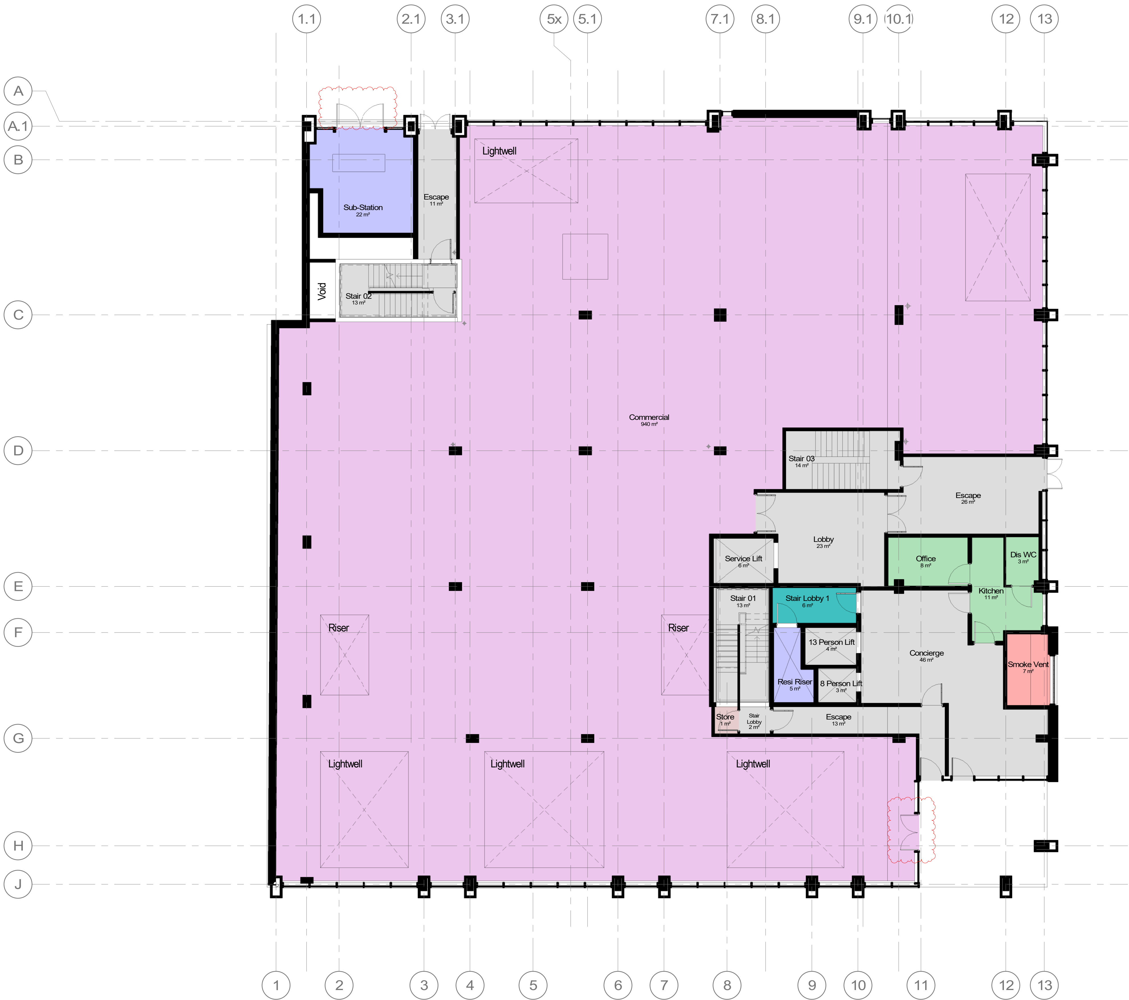
1 Ground Floor GA Plan 1 : 100
