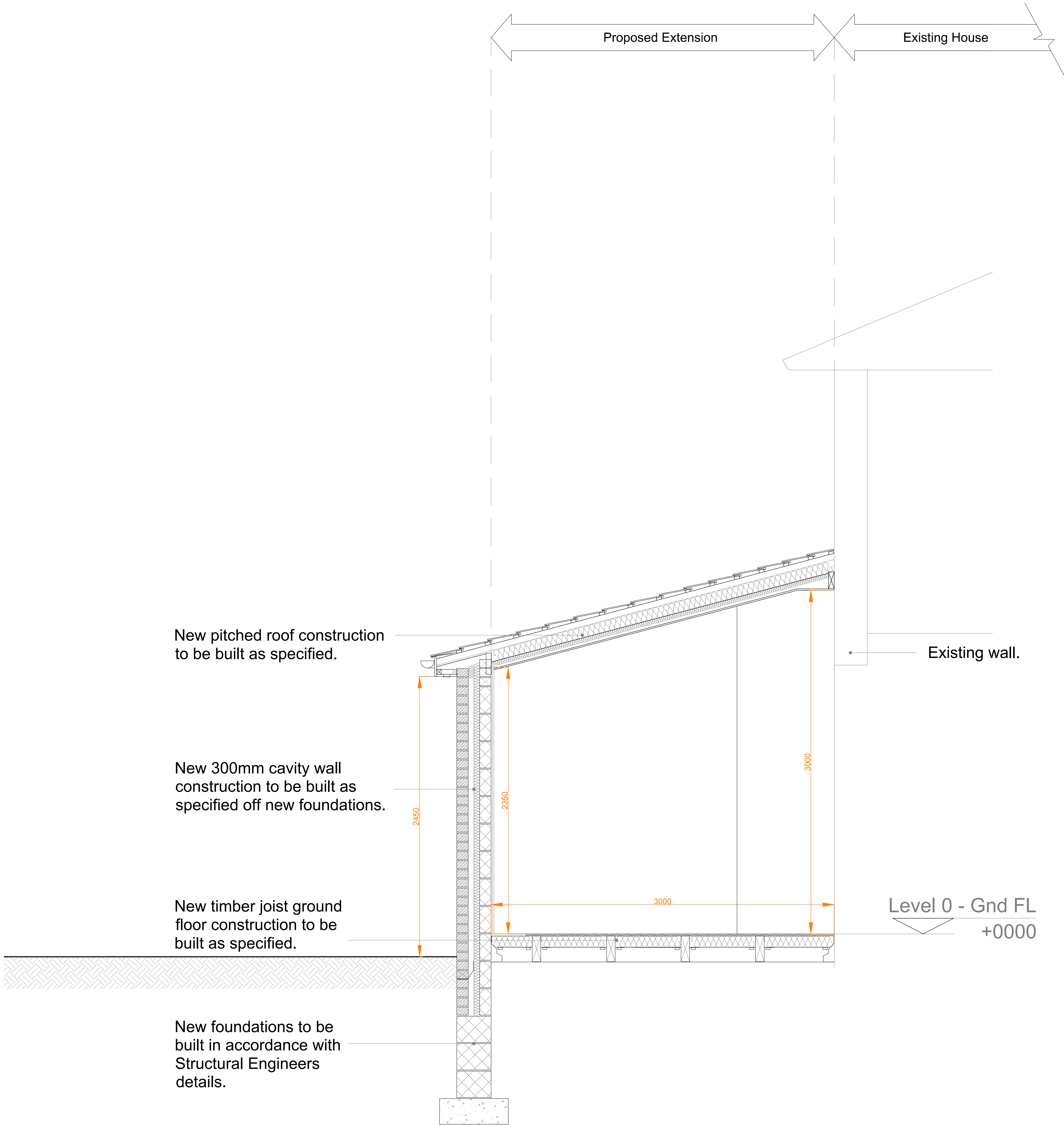
SECTION CC
