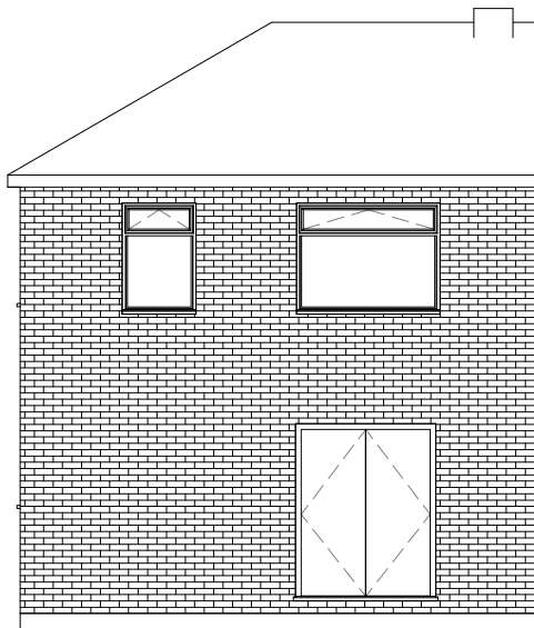
3 Rear Existing 1 : 100
