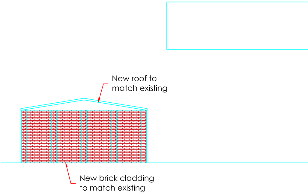
Proposed Garage Rear Elevation
