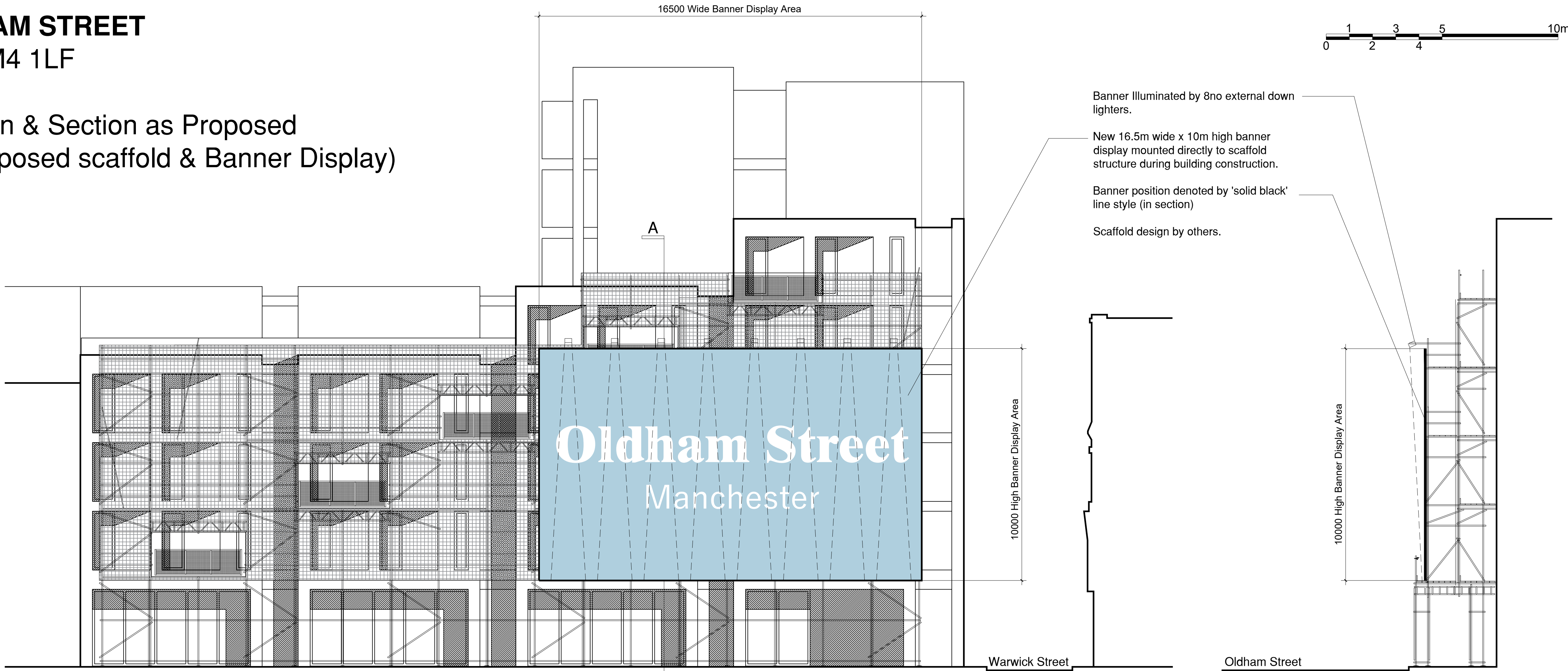
Banner Proposal: Oldham Street Elevation (including Construction Scaffold & Banner)
