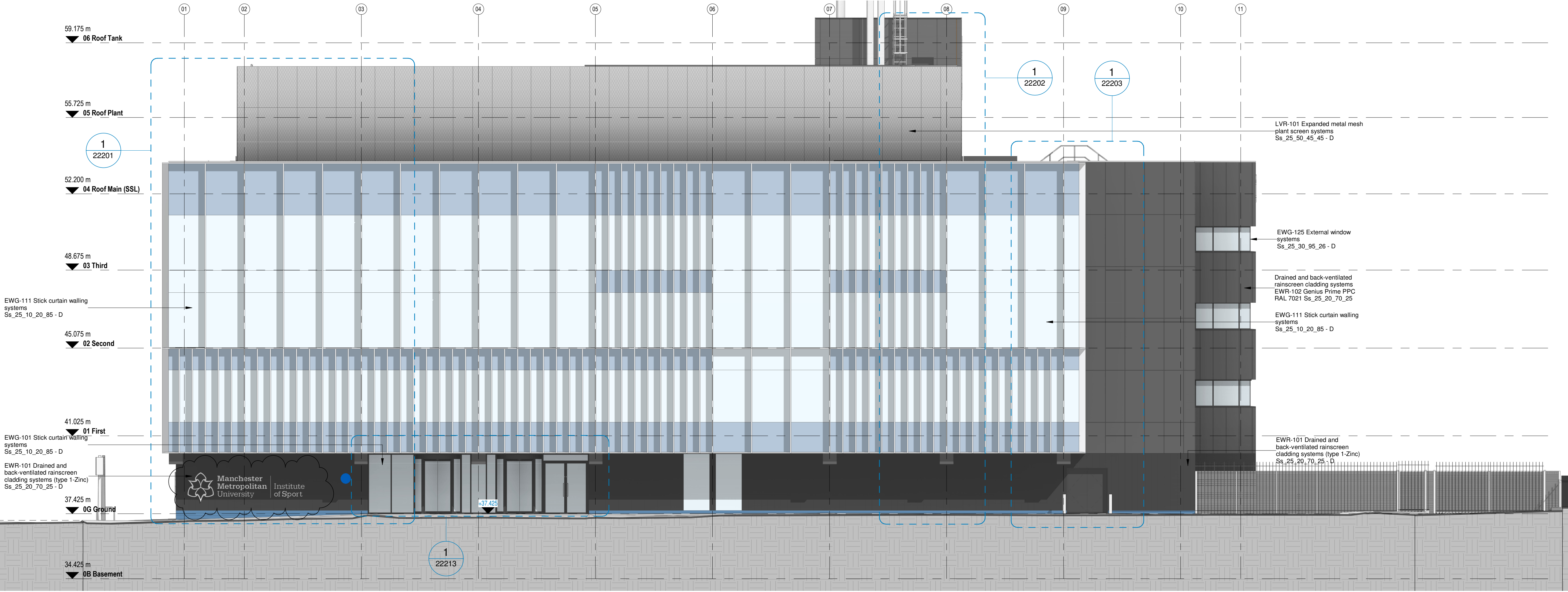
01 GA Elevation - Proposed South Sidney Street 1 : 100
