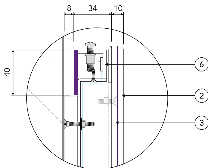
DETAIL B
