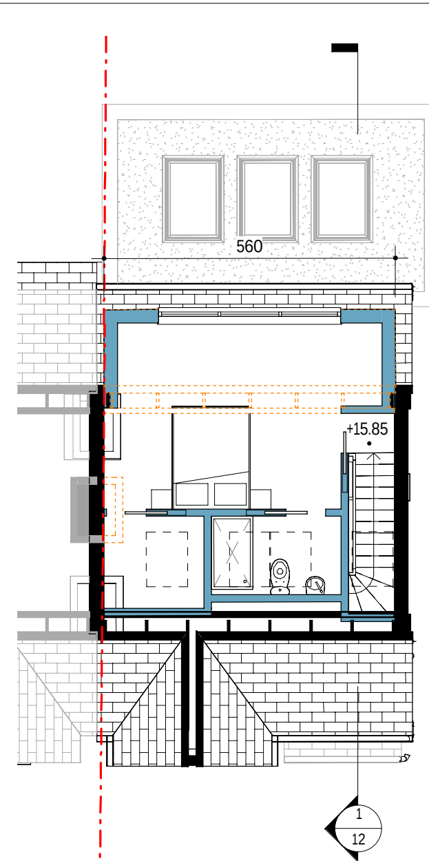
Proposed Loft 1 : 100
