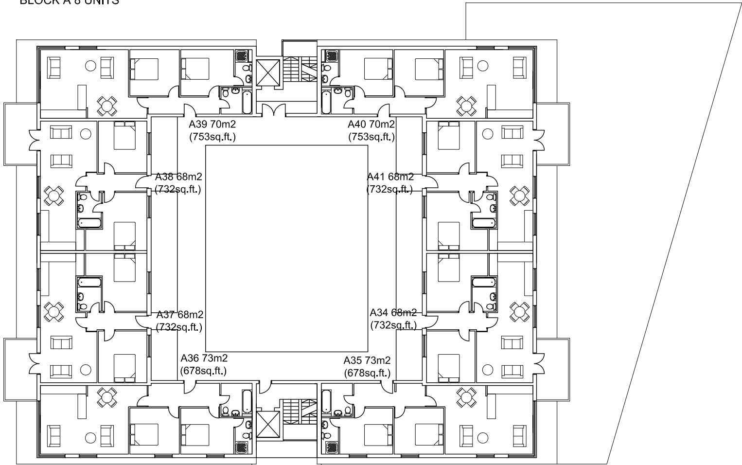
BLOCK A 8 UNITS
