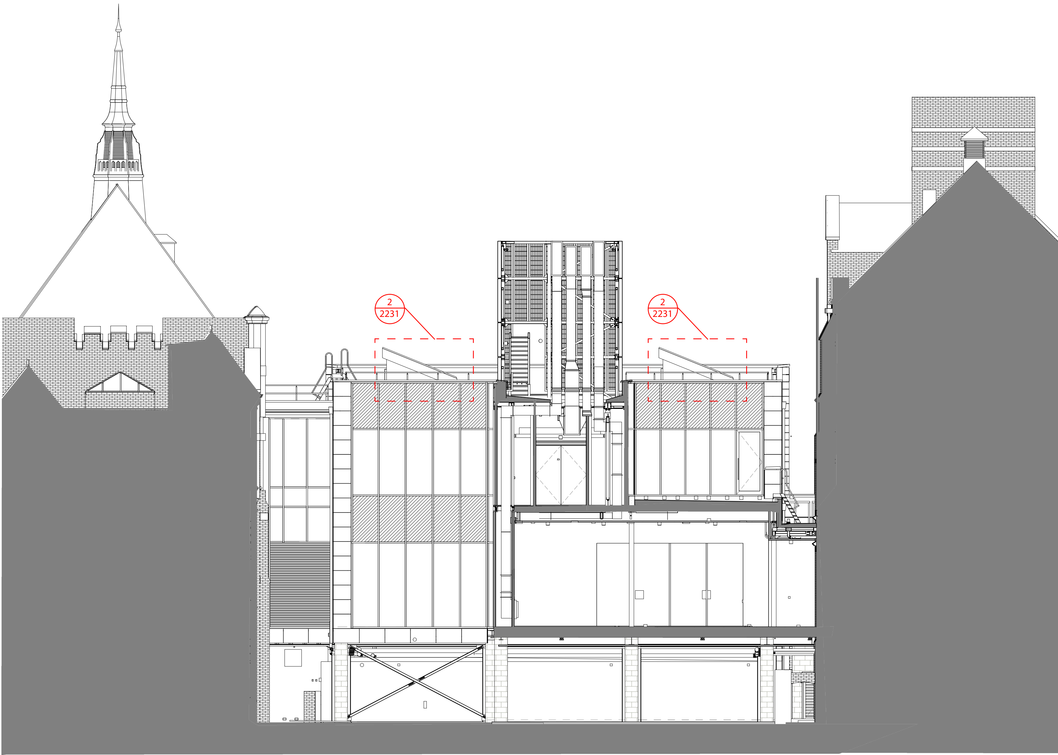
1 Louvres - Proposed Section GG 2231 1 : 100
