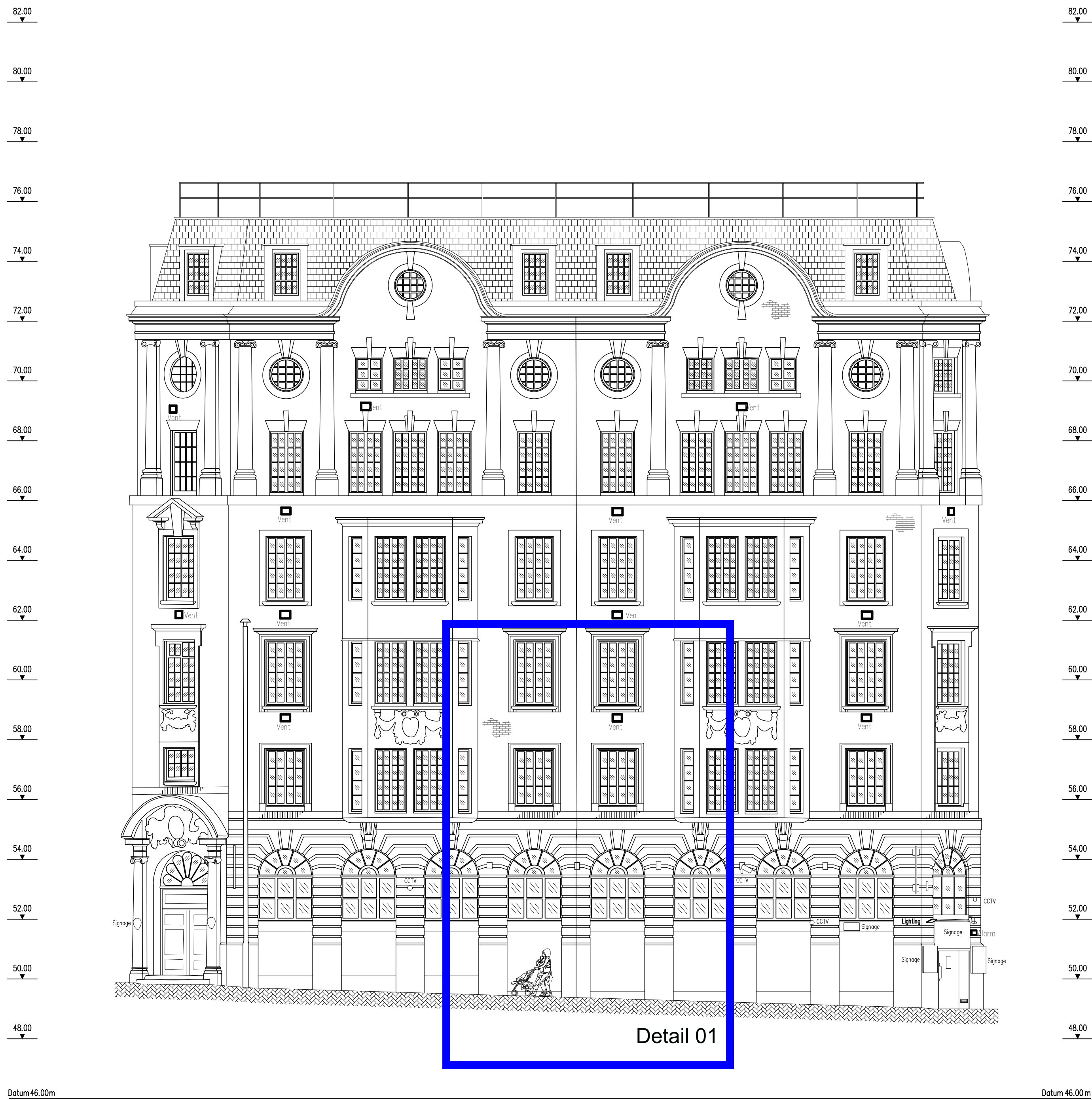
Proposed Elevation C
