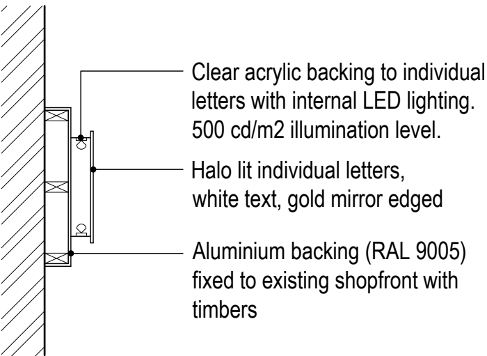
SECTION THRU' FASCIA SIGN 1:20
