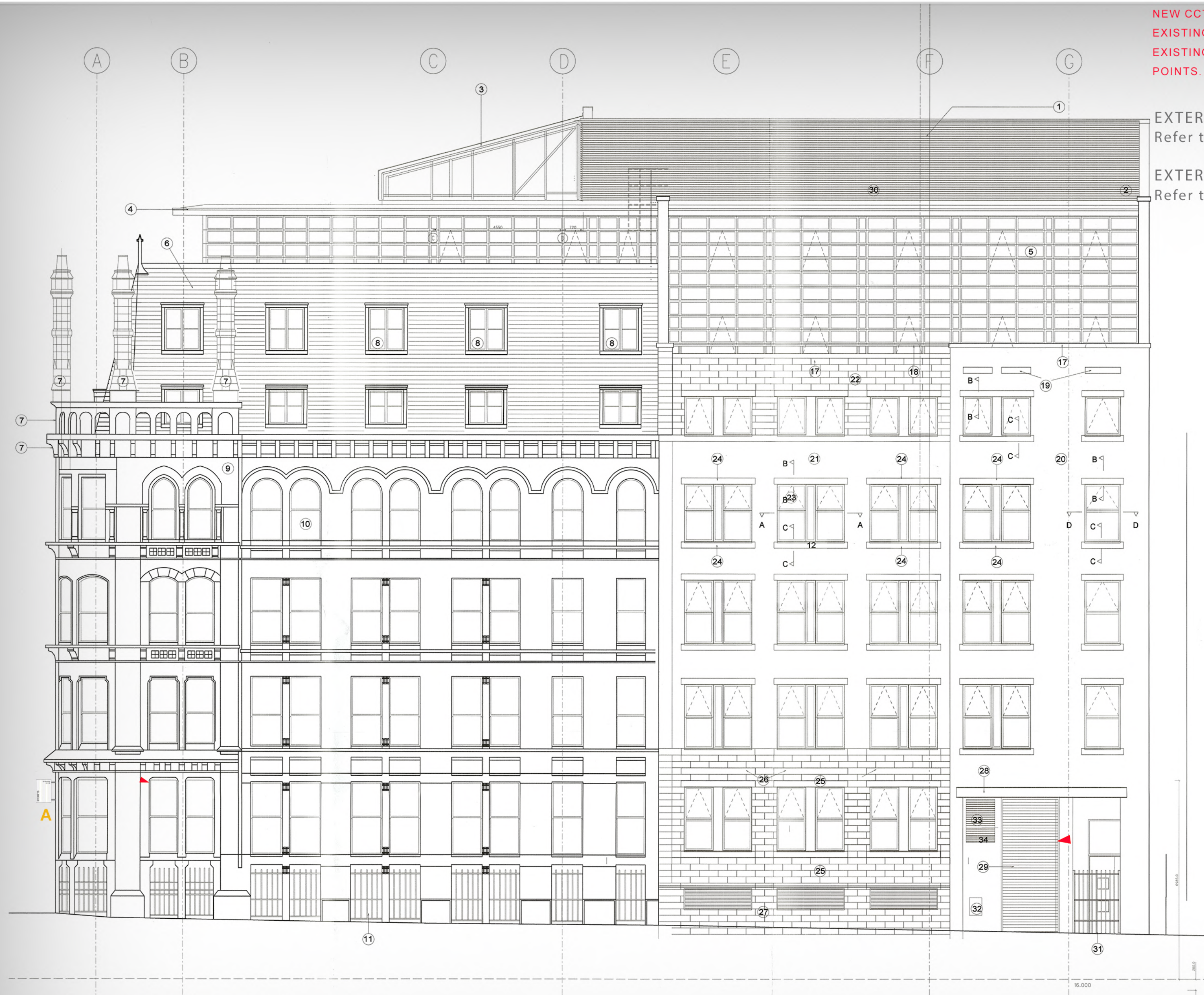
BACK GEORGE STREET ELEVATION
