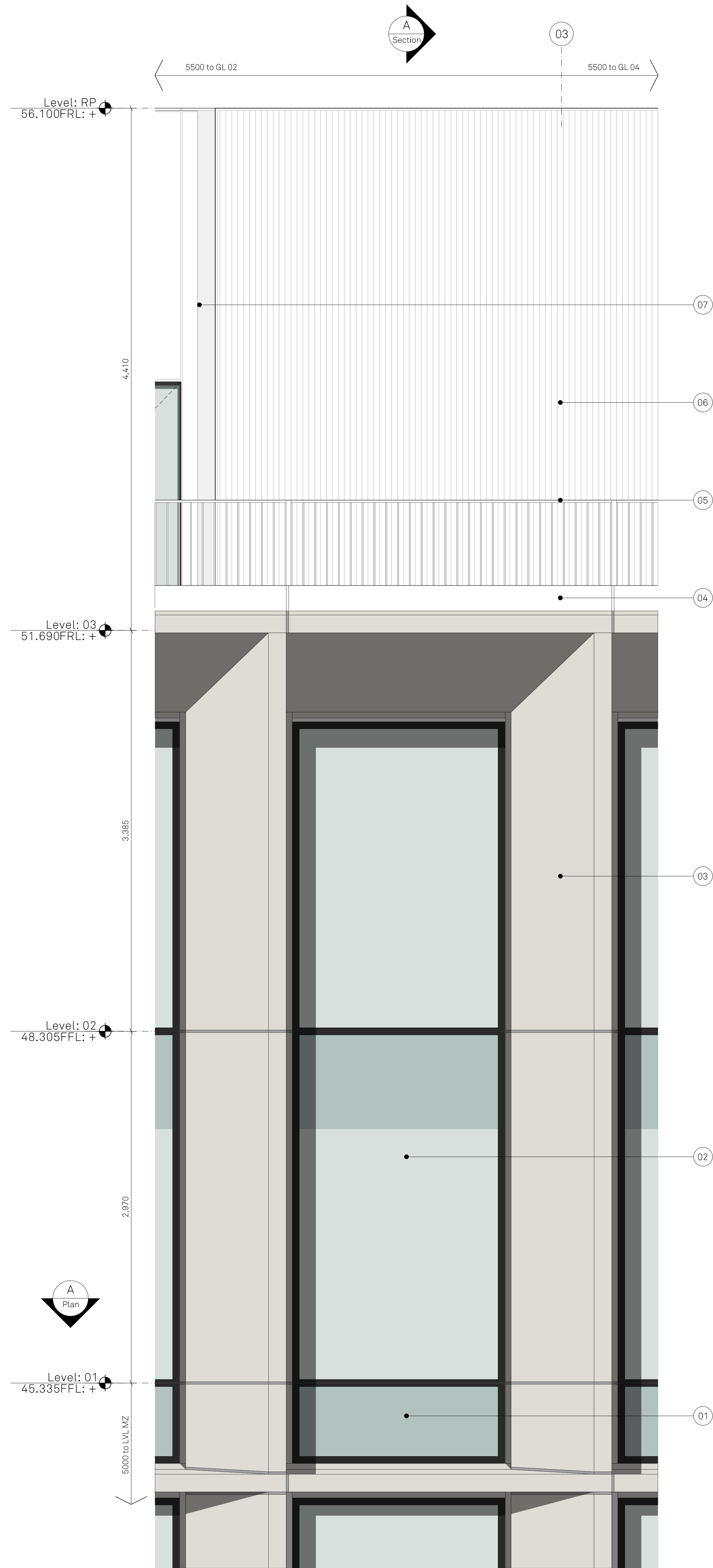
PARTIAL ELEVATION Typical Office Bay
