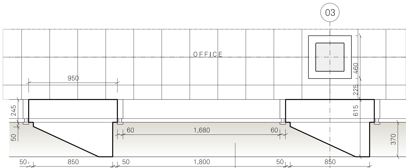
PARTIAL ELEVATION Typical Office Bay
