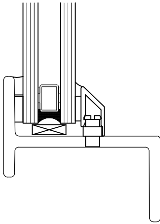
Section 1 - 1
