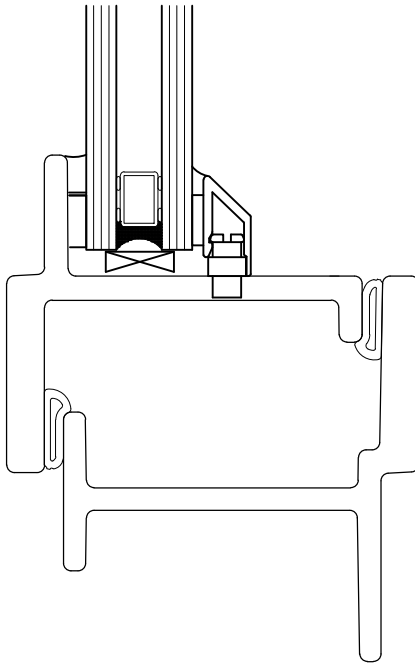
Section 2 - 2
