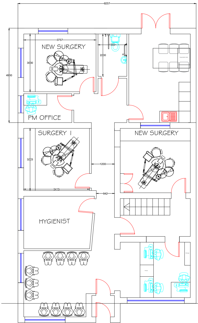
01 Proposed Ground Floor Plan 003 1:100 @ A3
