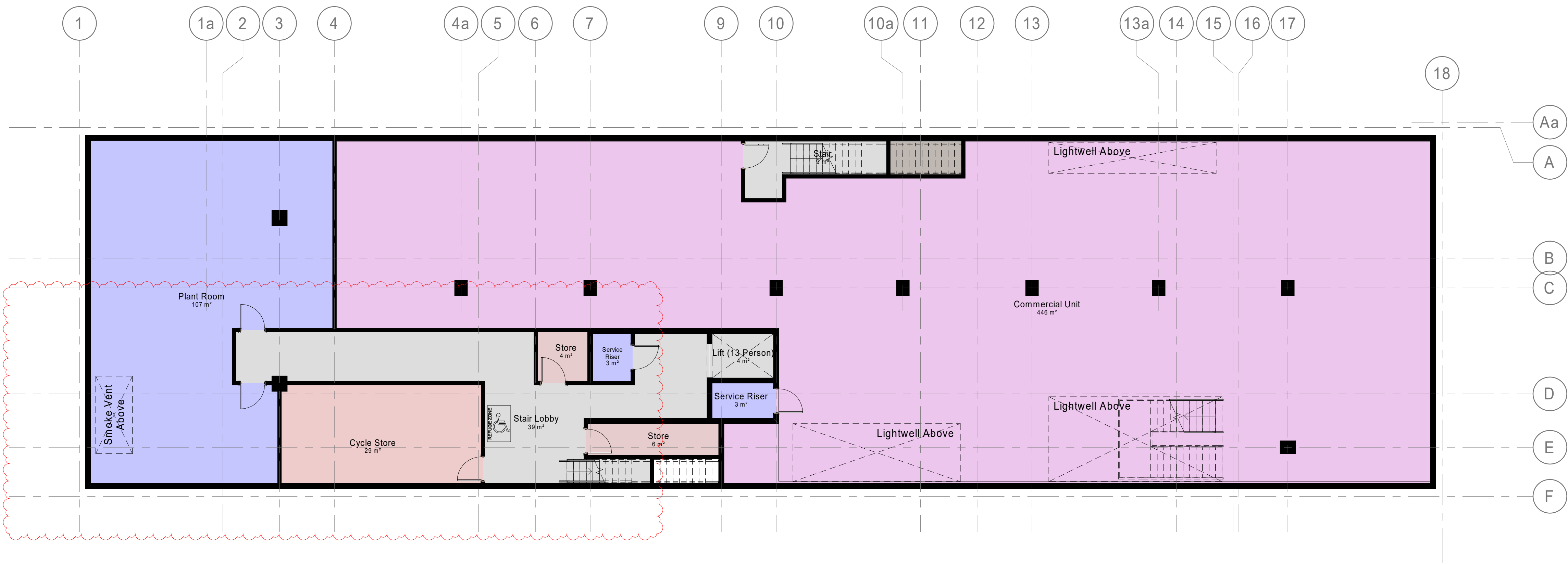
1 Lower Ground GA Plan 1 : 100
