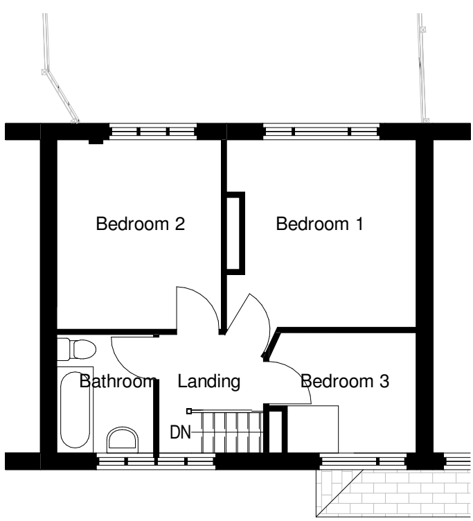
Level 1 Existing no. 12 1 : 100
