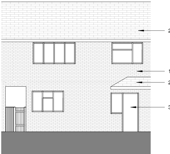
Existing Elevation North no. 12 1 : 100
