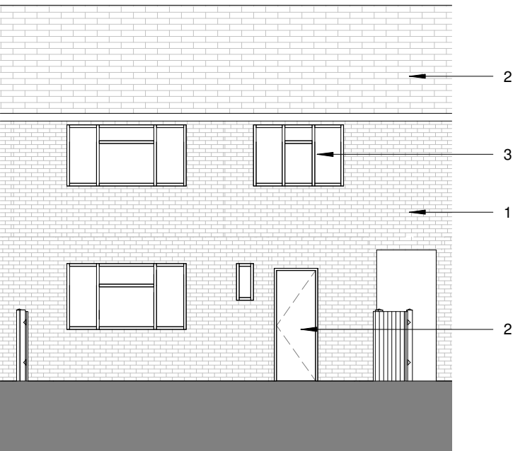
Existing Elevation South no. 12 1 : 100
