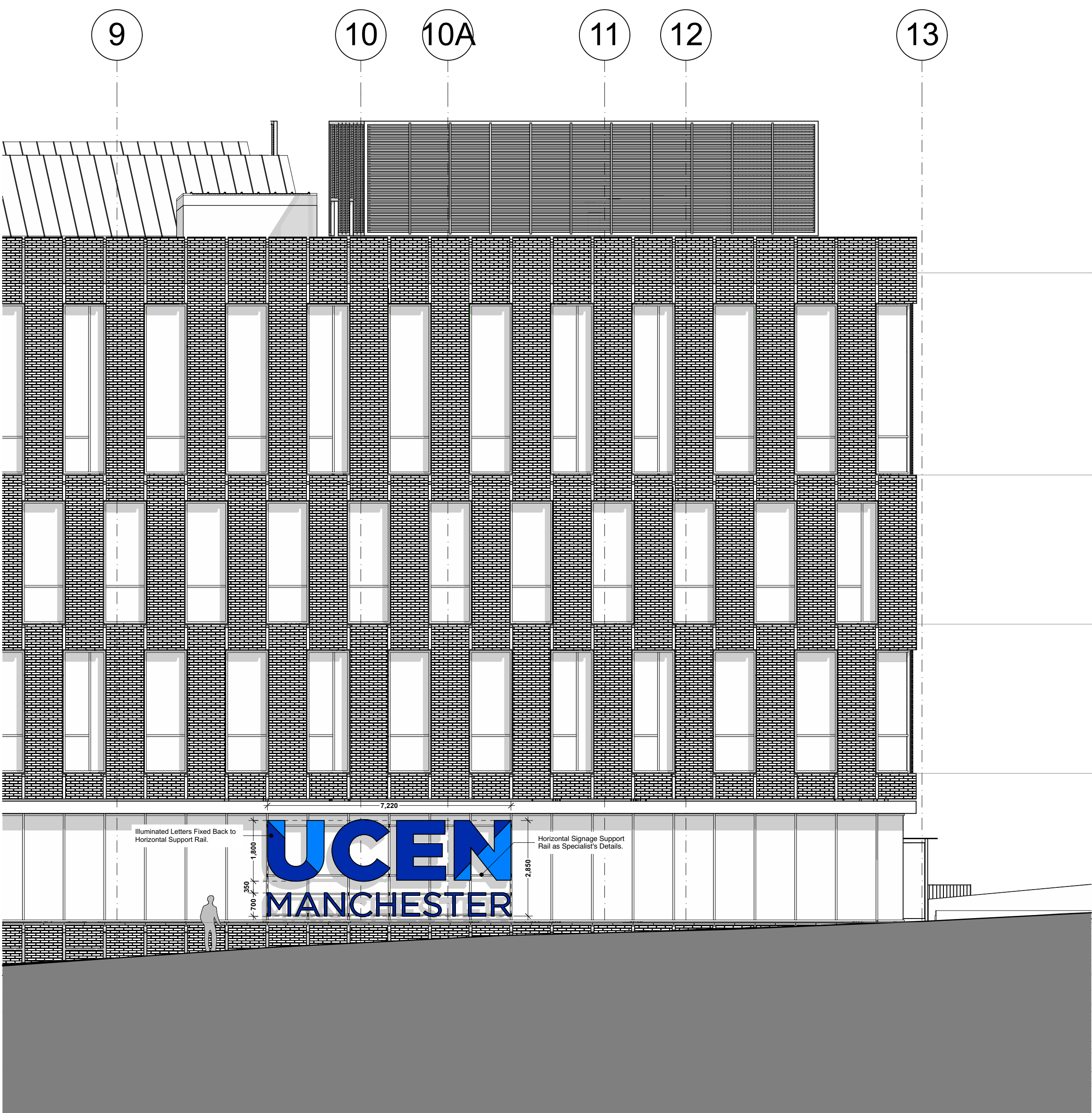
SIGN 3 - New Bridge Street - Elevation 1:100
