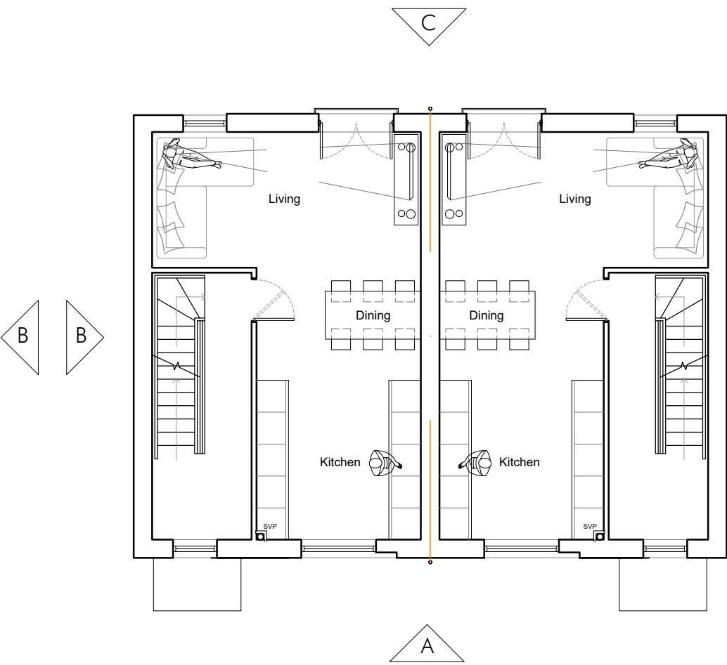
First Floor 38m 2 /418ft 2
