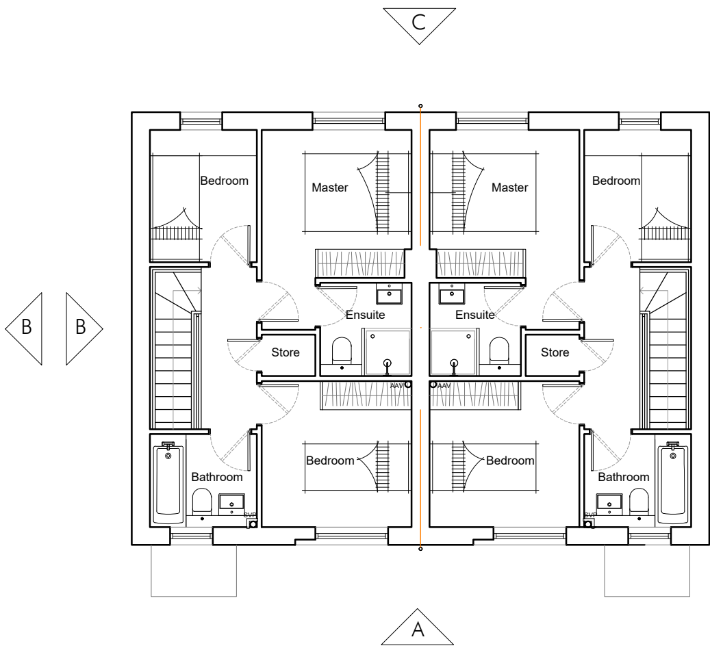
Second Floor 38m 2 /418ft 2
