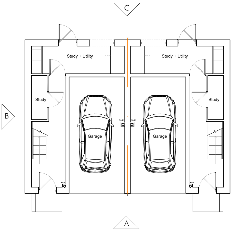
Ground Floor - ex Garage 19m 2 /206ft 2
