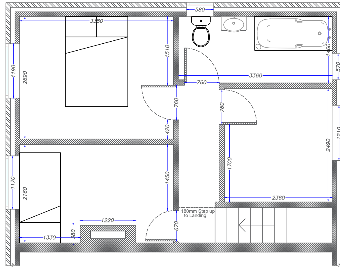
Existing 1st Floor Layout
