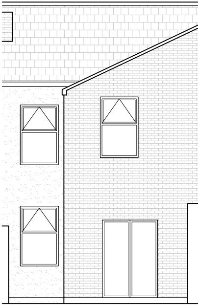
EXISTING REAR ELEVATION 1:100 @ A3
