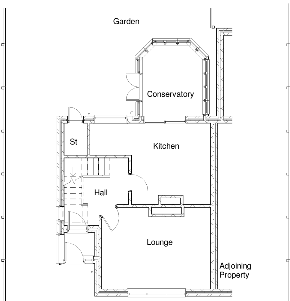
01 Existing Ground Floor Plan
