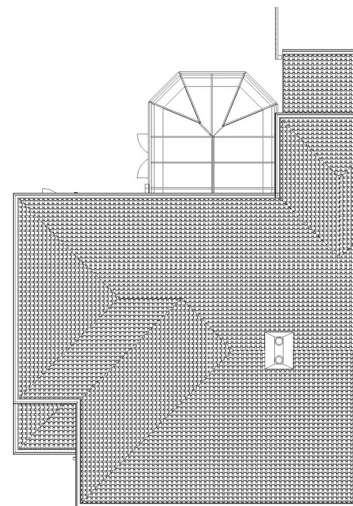
04 Existing Roof Plan
