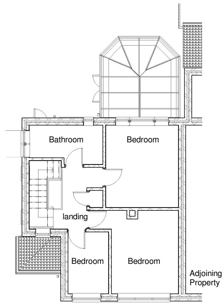
02 Existing First Floor Plan
