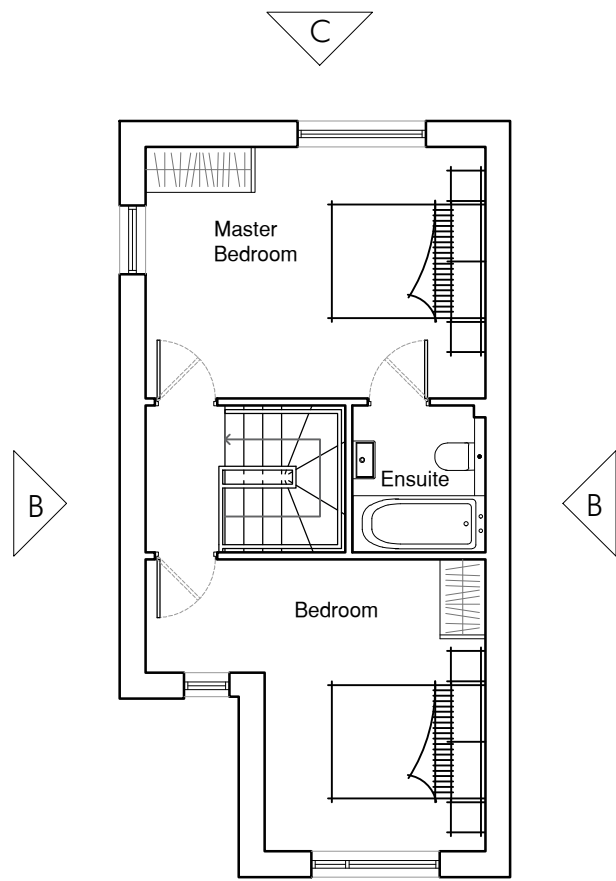
Second Floor 38m²/411ft²
