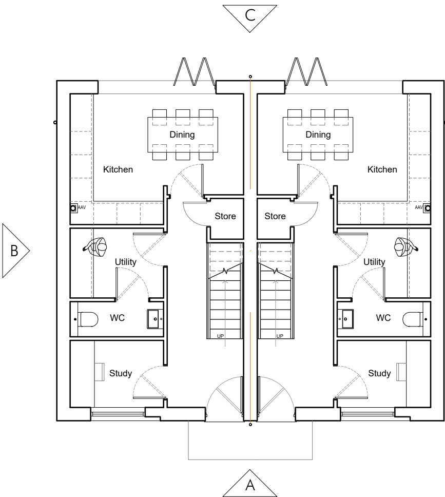
Ground Floor 36m 2 /388ft 2
