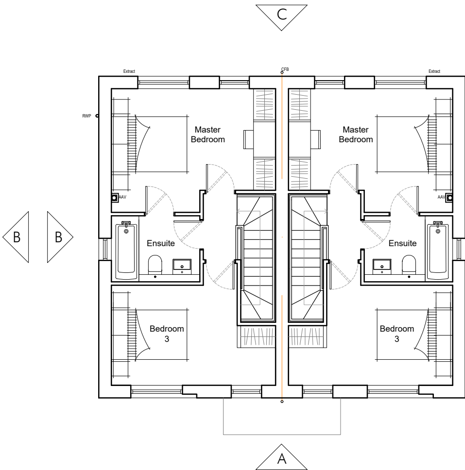
Second Floor 36m 2 /388ft 2
