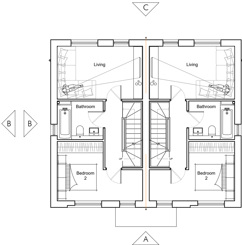
First Floor 36m 2 /388ft 2
