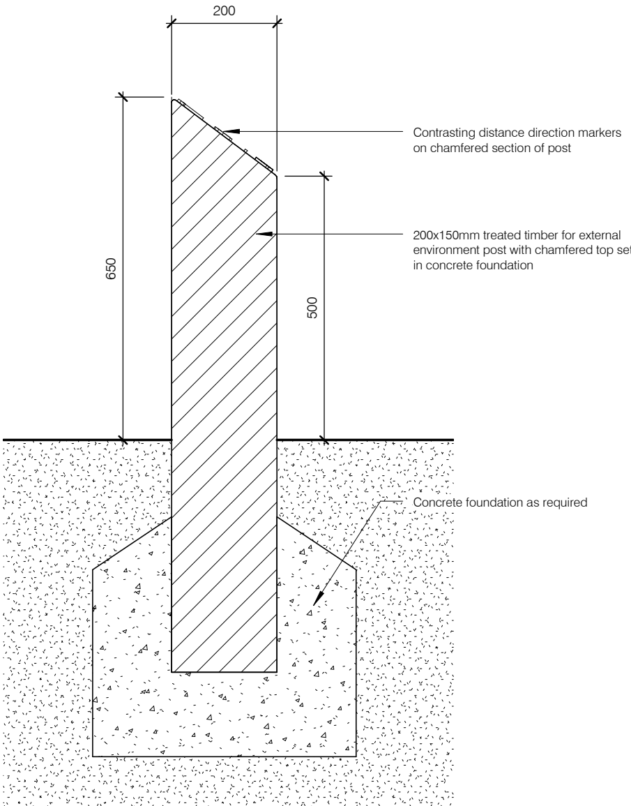
Run-Loop Markers - Section
