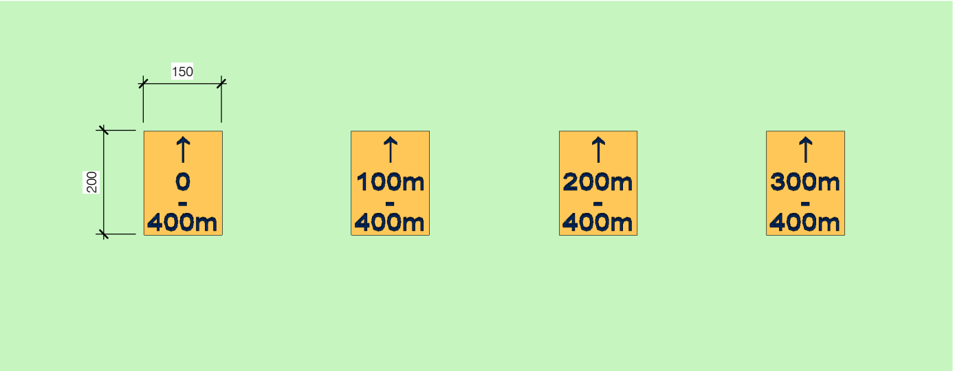
Run-Loop Markers - Plan
