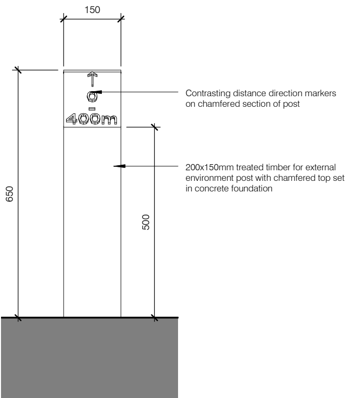
Run-Loop Markers - Elev
