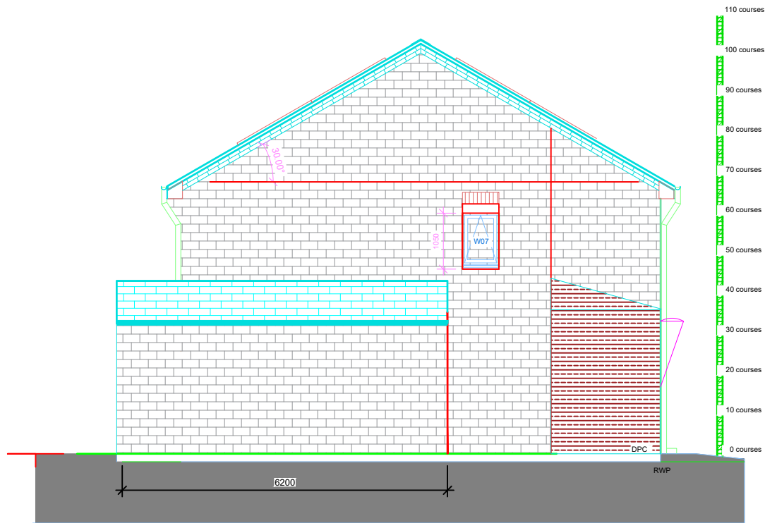
1 Existing Side A Elevation 1 : 100 @ A3
