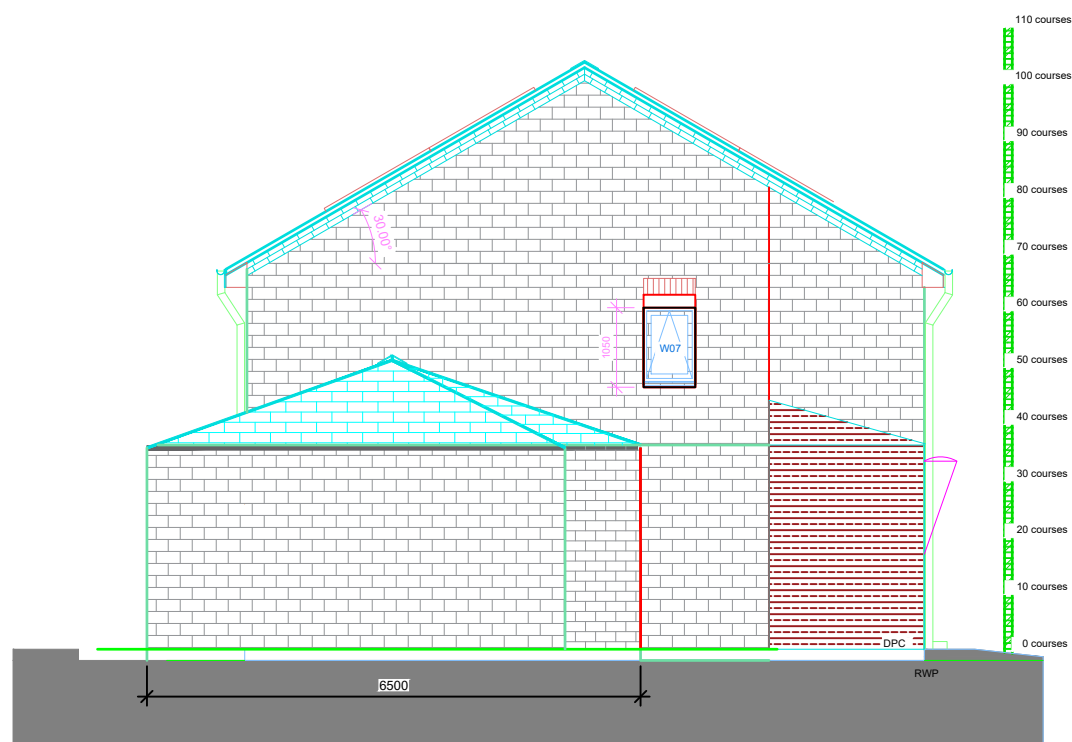
2 Proposed Side A Elevation 1 : 100 @ A3
