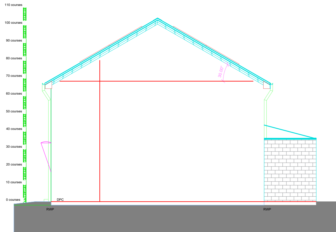
3 Existing Side B Elevation 1 : 100 @ A3
