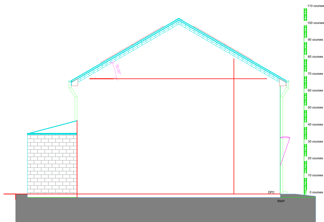
4 Proposed Side B Elevation 1 : 100 @ A3
