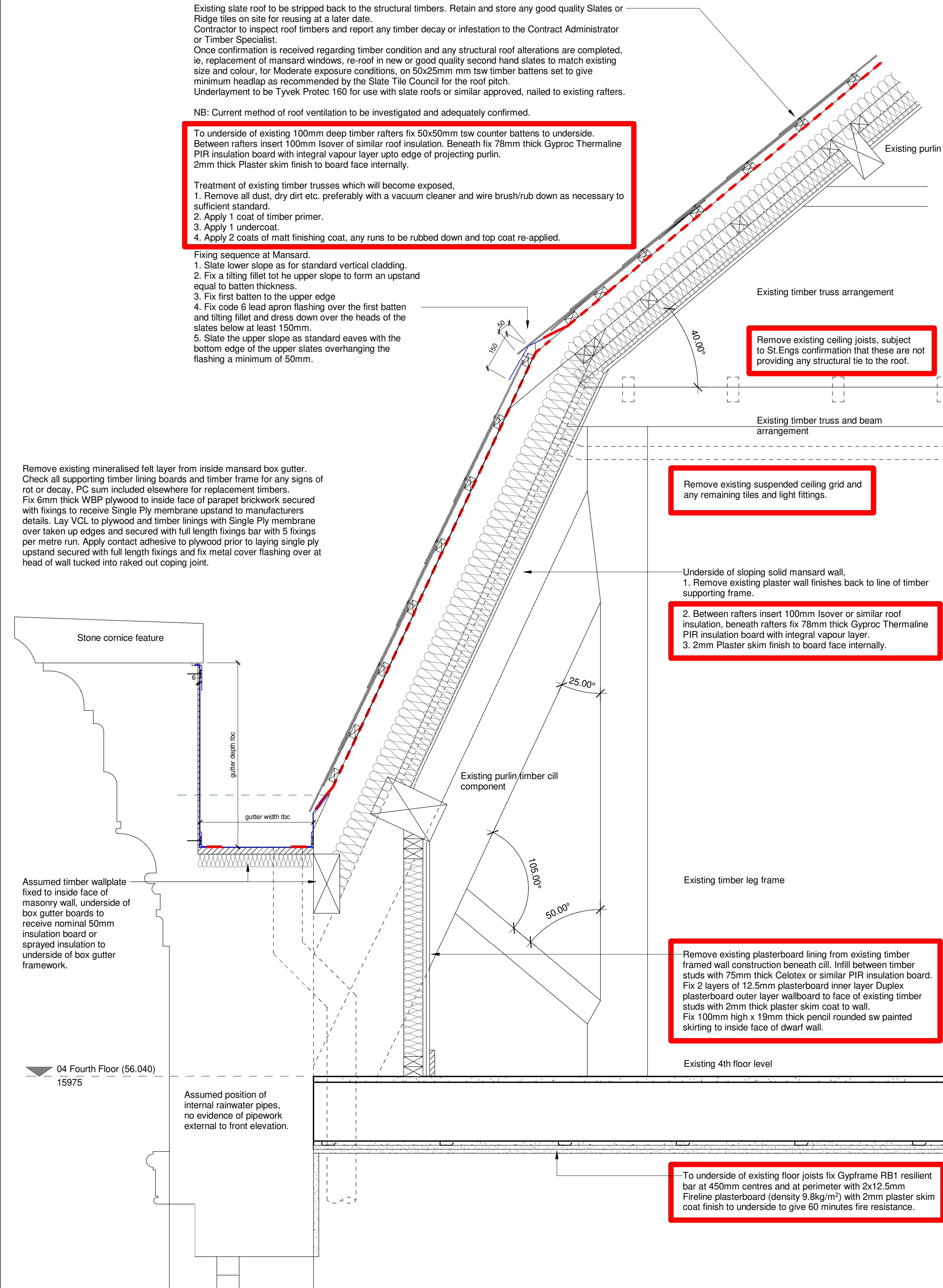
Proposed section thro' Mansard Roof 1 : 10
