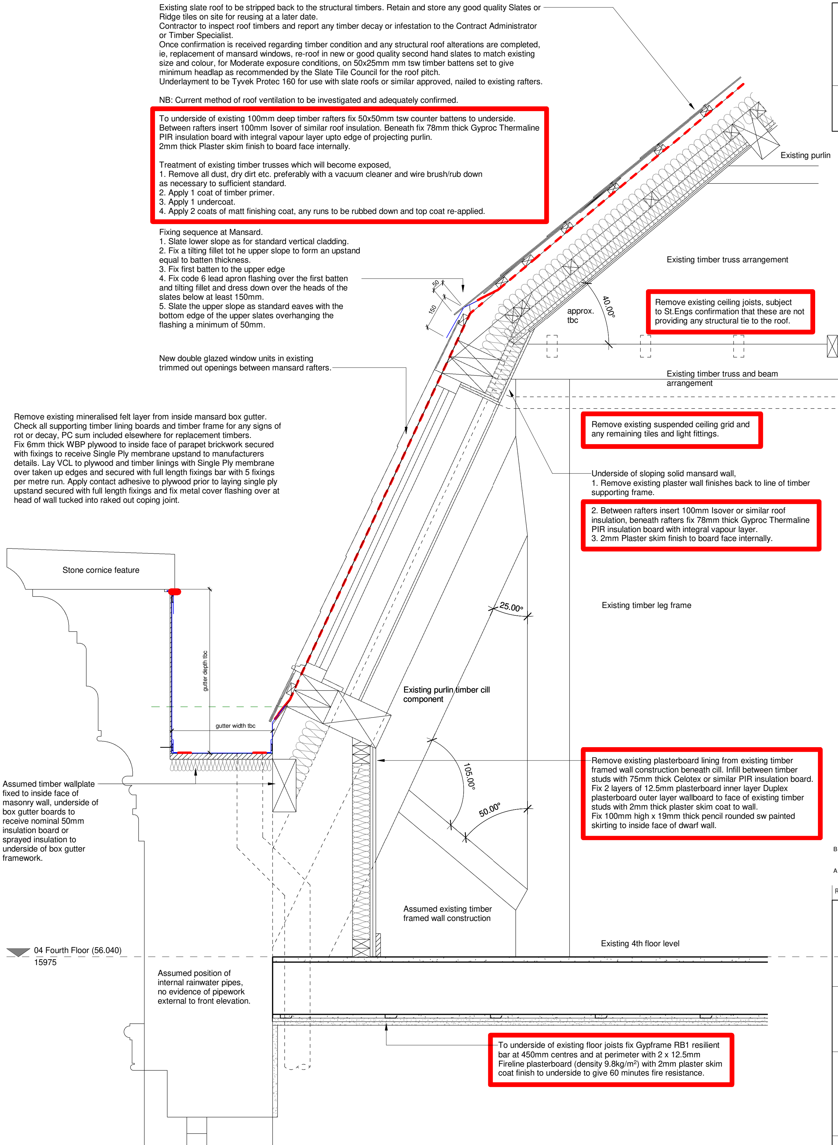
Proposed section thro' Window Mansard Roof 1 : 10
