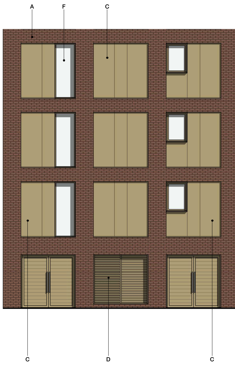
Extract 1 of Elevation D 1 : 100
