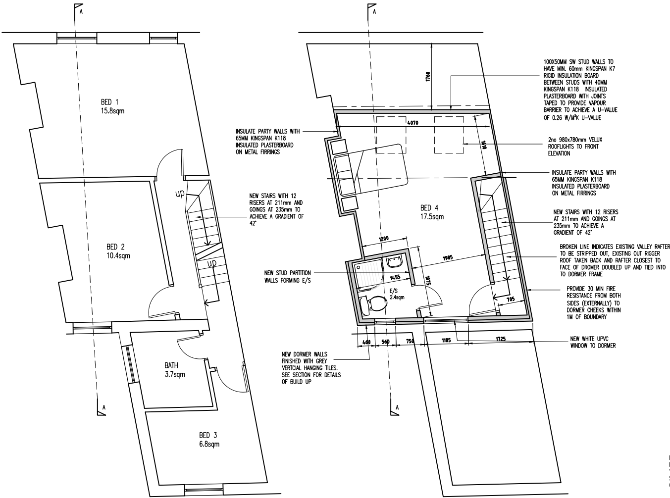
PROPOSED SECOND FLOOR PLAN 1:100 @ A3
