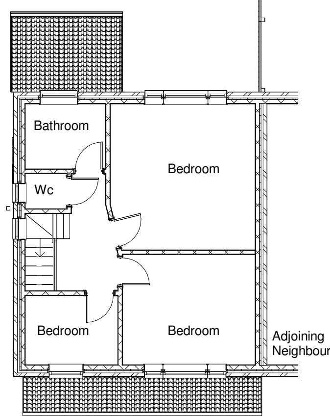
02 Existing First Floor Plan 1 : 100
