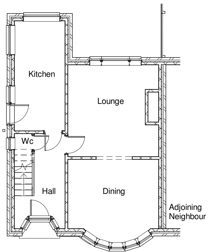
01 Existing Ground Floor Plan 1 : 100
