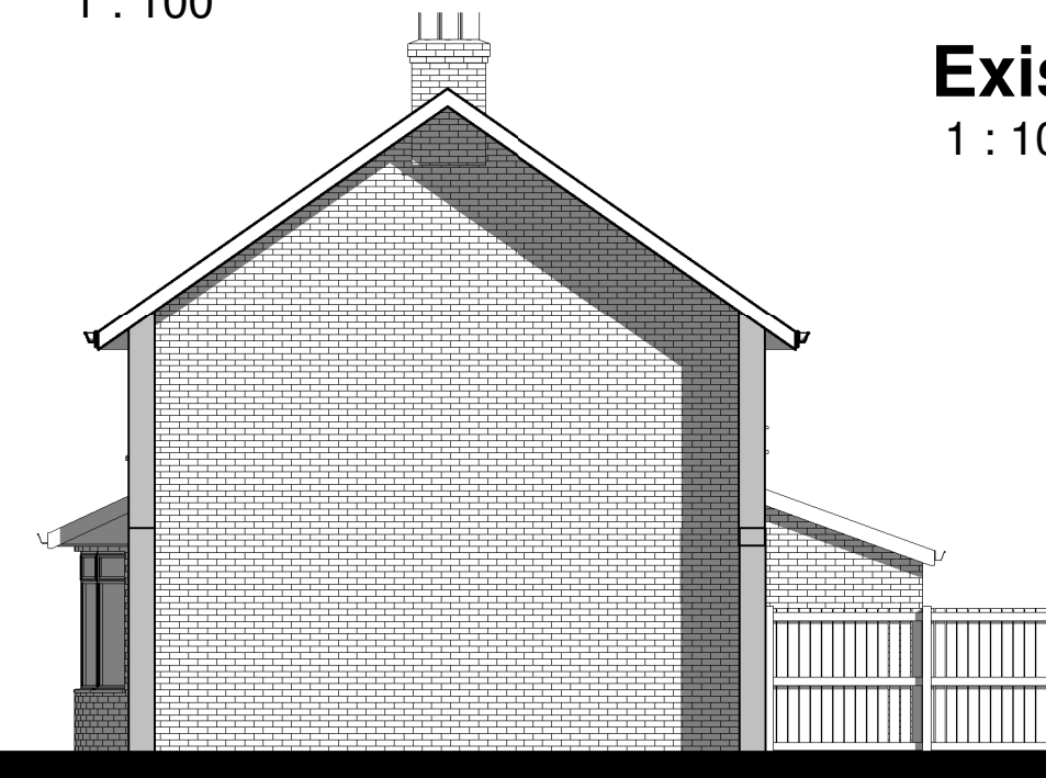
Existing Side Elevation 1 1 : 100
