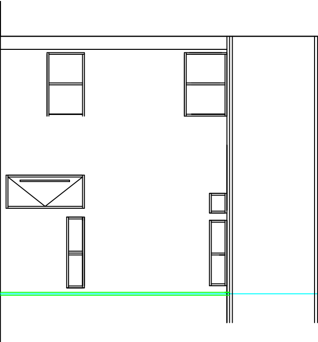
EXISTING FRONT VIEW 1:100
