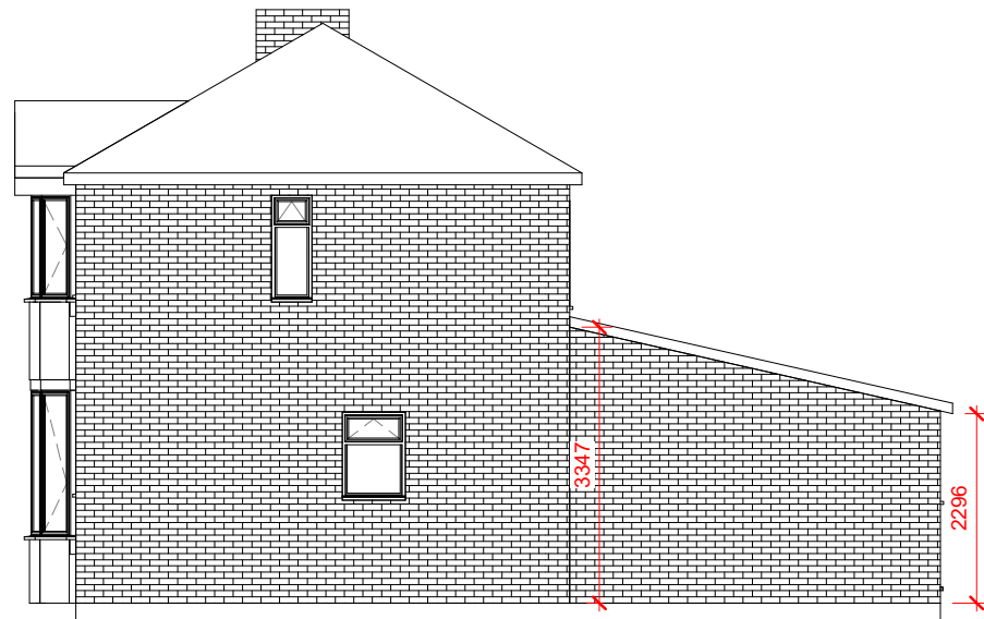
4 Right Proposed 1 : 100
