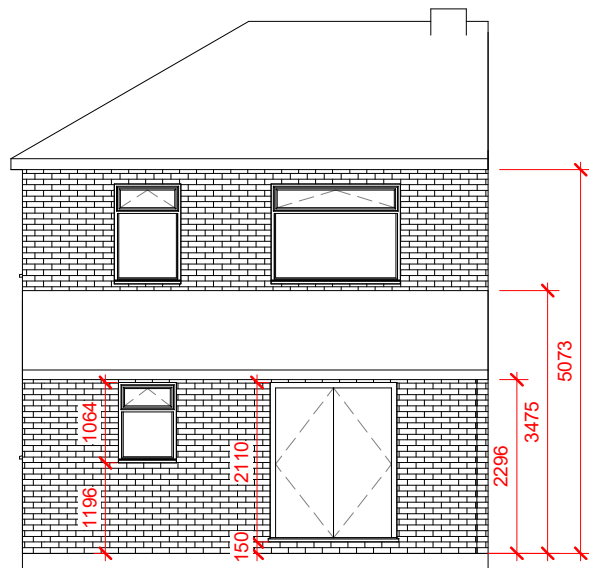
3 Rear Proposed 1 : 100
