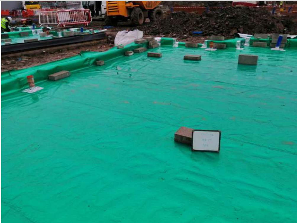
Photograph 5: Validation of Gas Membrane Installation
