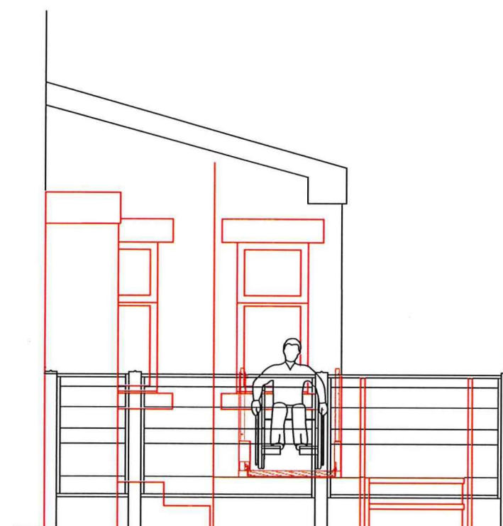
PROPOSED SIDE ELEVATION VIEWED FROM ADJOINING PROPERTY
