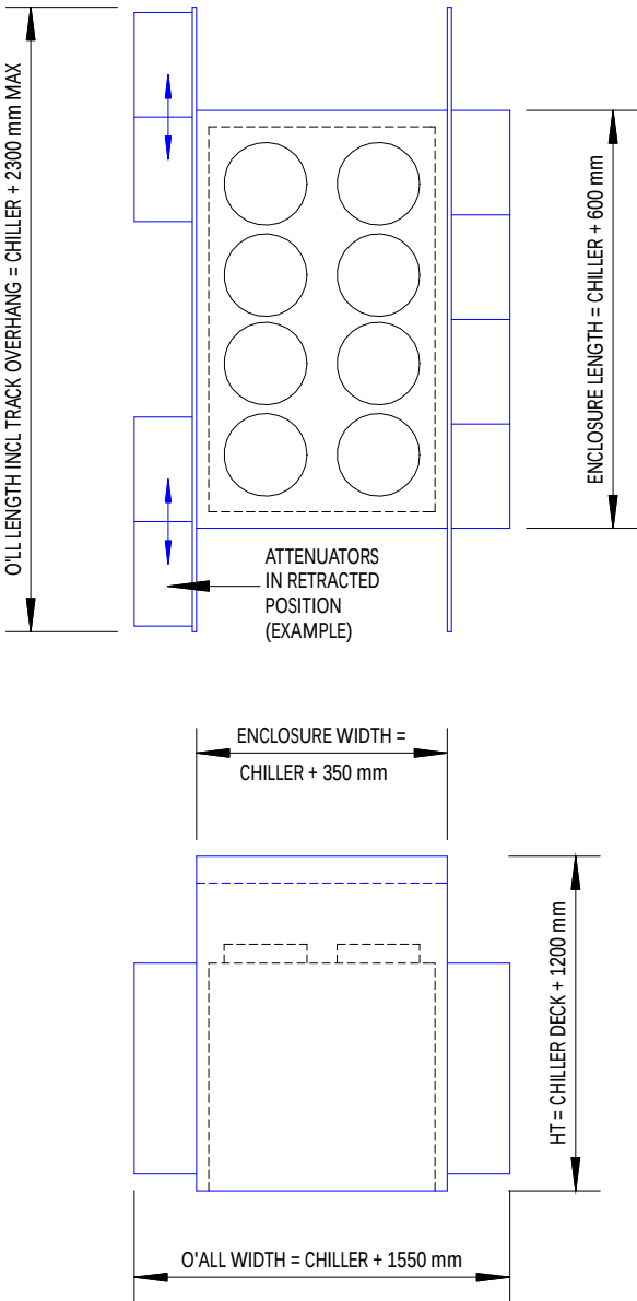
INCREASE IN DIMENSIONS OF BASE CHILLER (NOMINAL)
