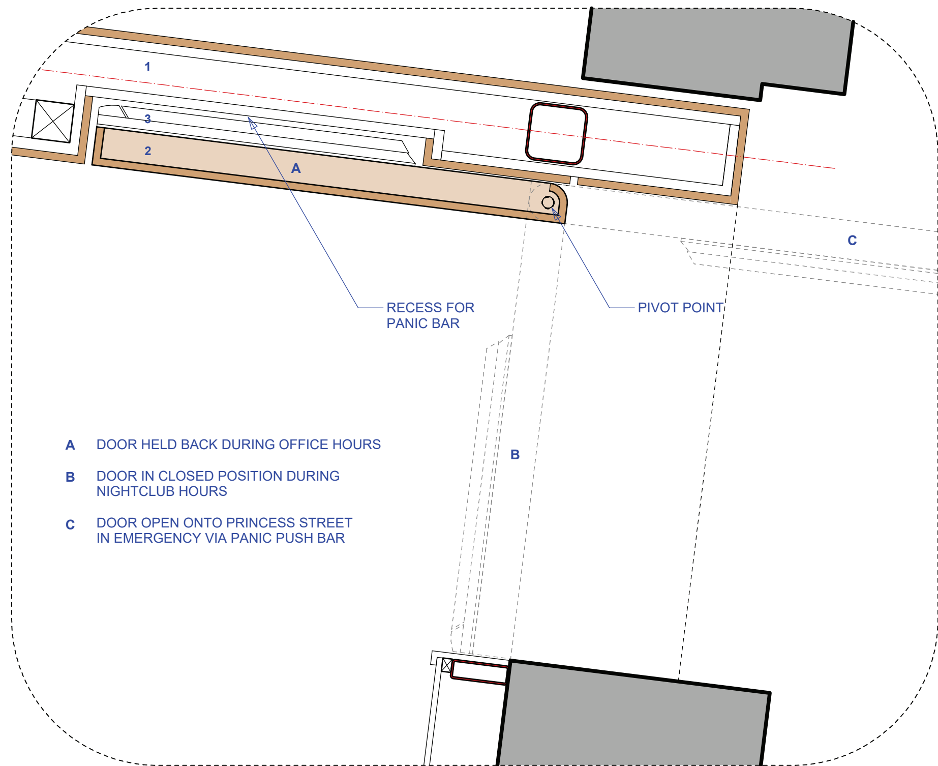
CALL OUT DETAIL TO DOOR (1:10)
