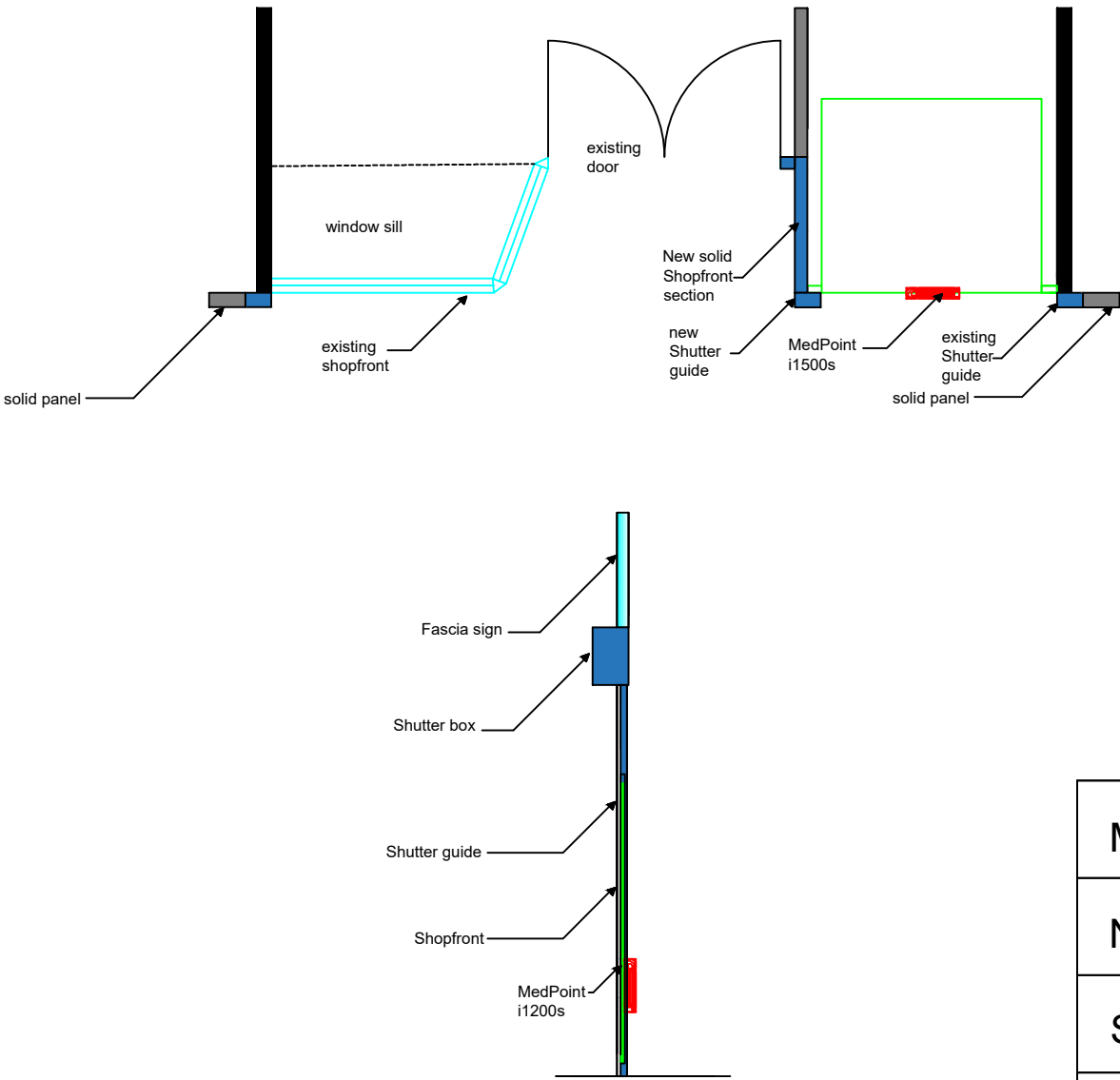
Proposed Shopfront - side elevation
