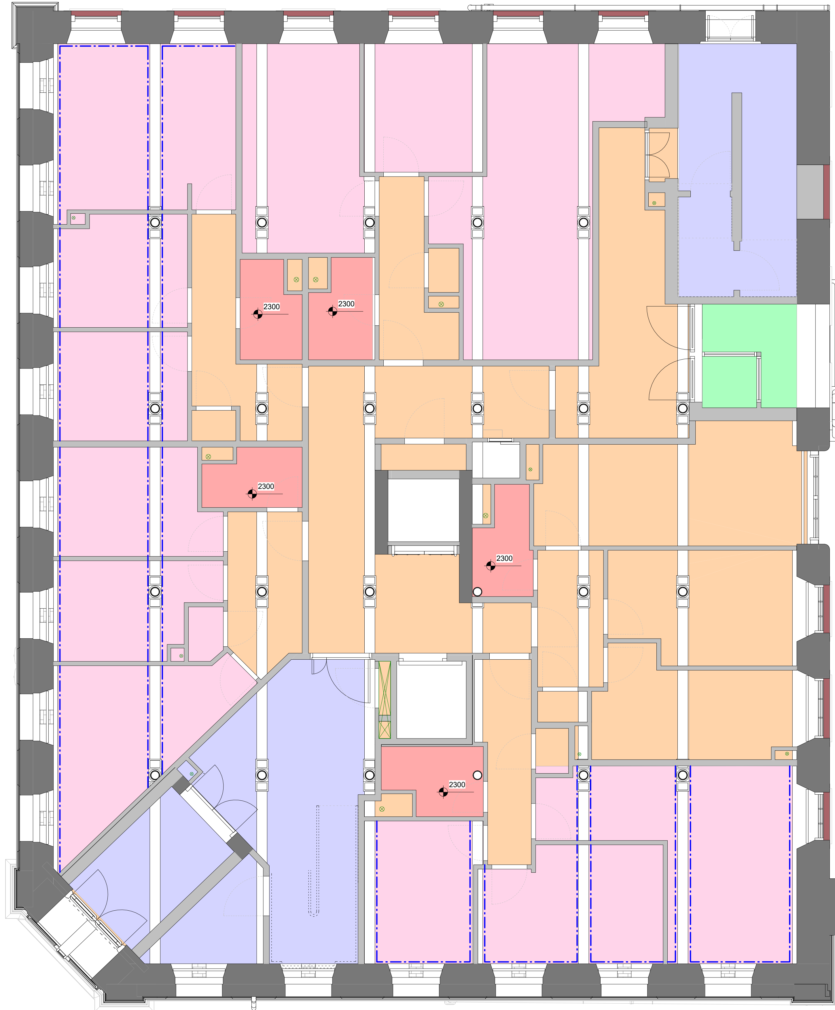
1 00 - GROUND FLOOR - REFLECTED CEILING PLAN 1:50
