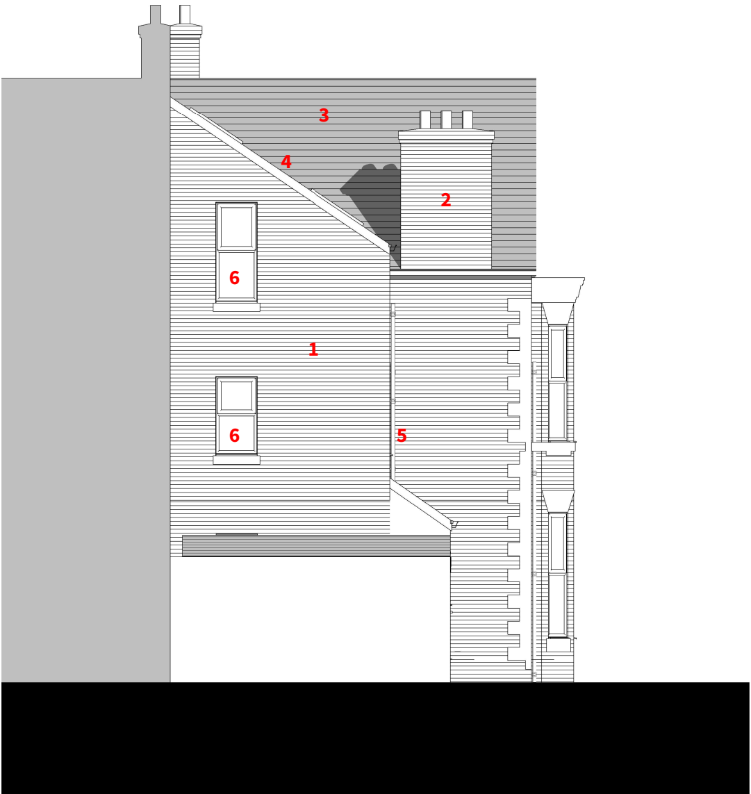
Existing Side Elevation A
