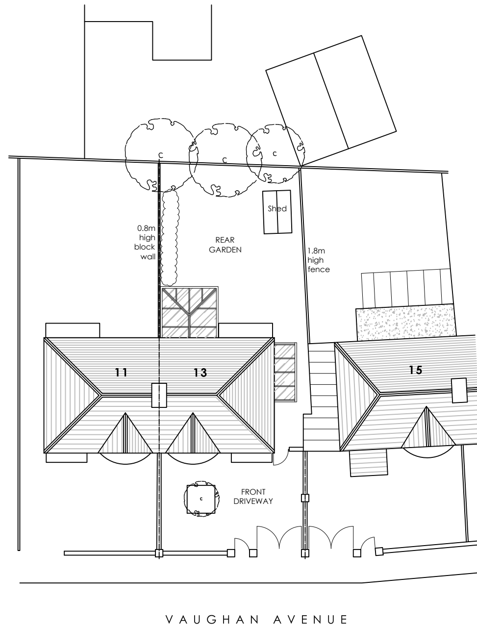
SITE / ROOF PLAN AS EXISTING 0 2m 4m 6m 8m 10m SCALE
