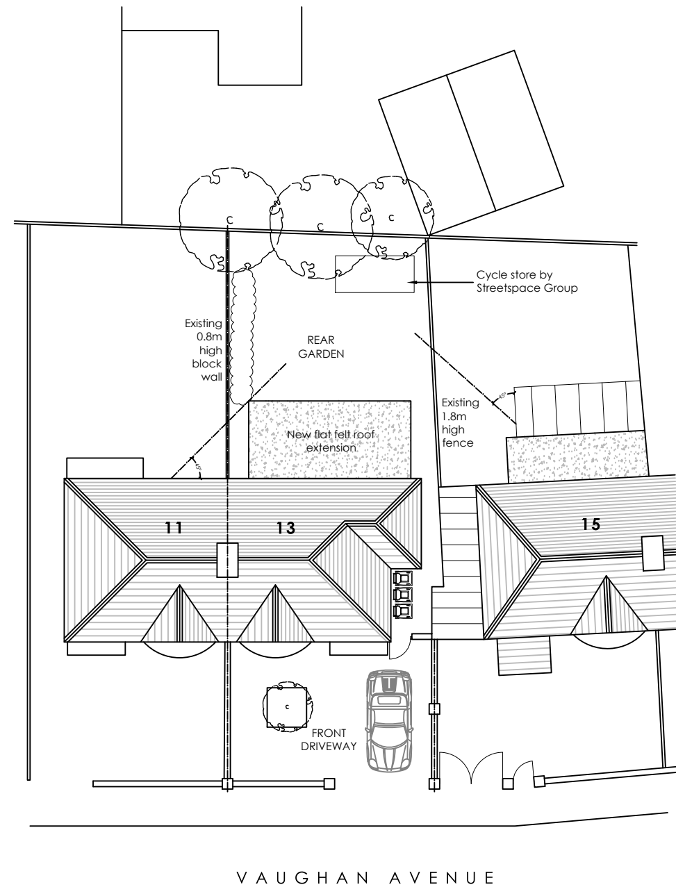
SITE / ROOF PLAN AS PROPOSED 0 2m 4m 6m 8m 10m SCALE
