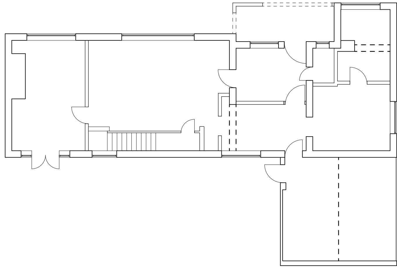
GROUND FLOOR SCALE 1:100 EXISTING - E003
