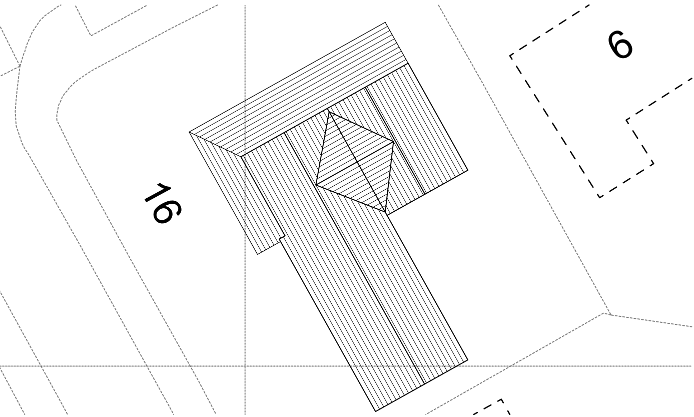
ROOF PLAN SCALE 1:200 UID - P001
