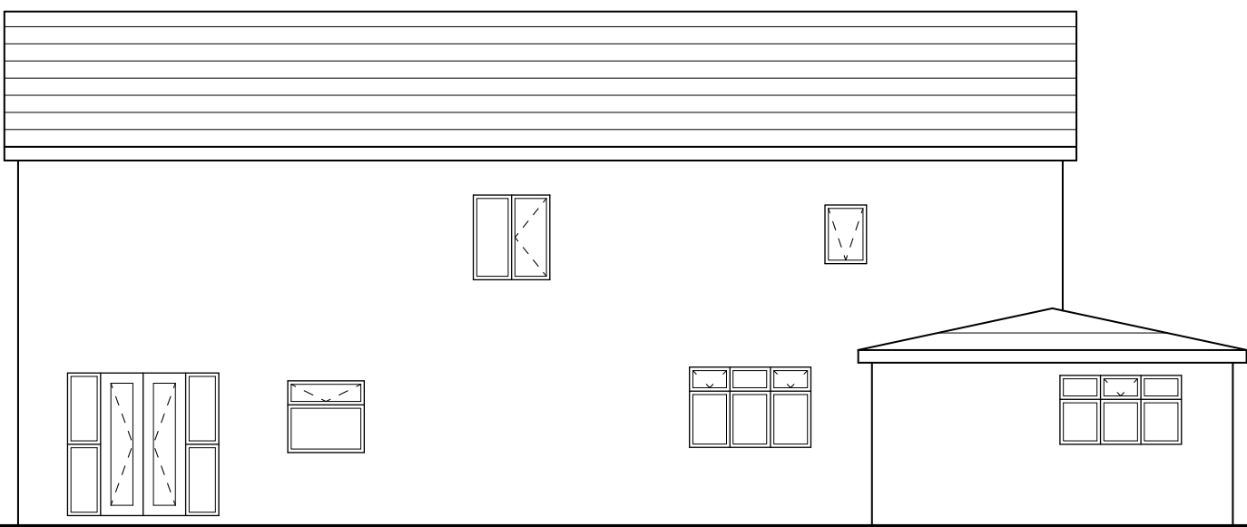
SOUTH EAST ELEVATION SCALE 1:100 EXISTING - E007
