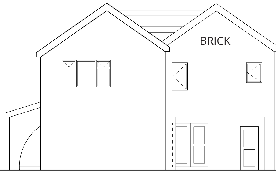
SOUTH WEST ELEVATION SCALE 1:100 PROPOSED - P009
