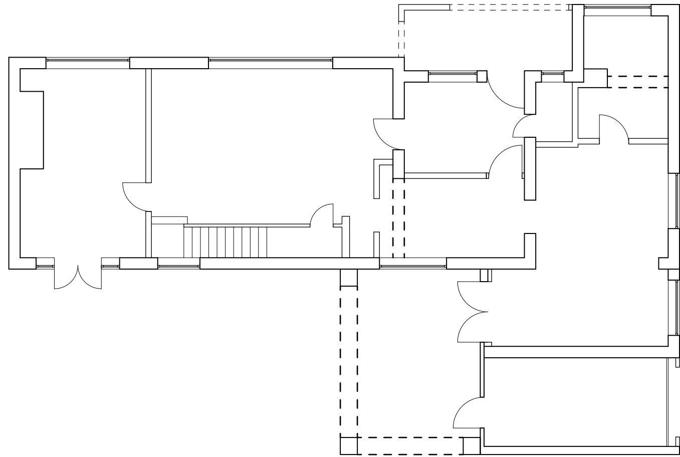
GROUND FLOOR SCALE 1:100 PROPOSED - P003
